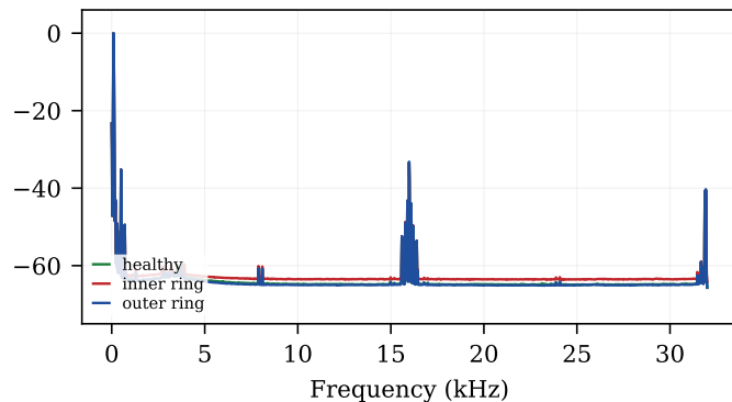
(c) Paderborn, as recorded 3 classes, many specimens
