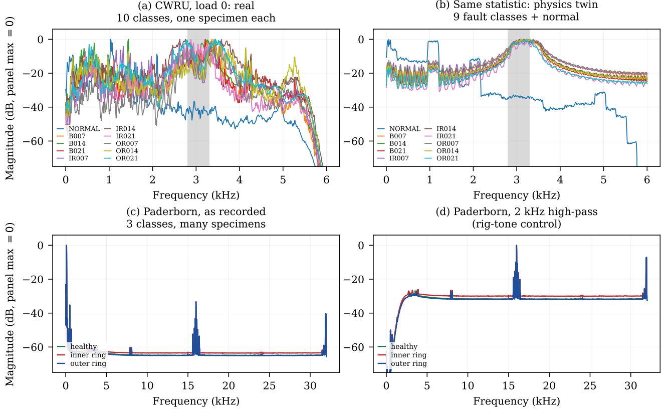
Fig. 2. Class-mean magnitude spectra under the identical, unsmoothed statistic of Table IV. Each panel is normalized to its own maximum (0 dB); all four share the same -75 dB floor, the same linear frequency axis and the same per-class colours, and the shaded span marks the 2800–3300 Hz band whose energy fraction is quoted in Section V. (a) CWRU, ten classes, one physical specimen each: visibly separated. (b) The physics twin, same statistic: the nine fault classes collapse into one band. Their median pairwise separation is 2.5 dB (minimum 0.9 dB), against 6.7 dB (minimum 3.7 dB) for the nine real classes, and across frequency the nine twin curves span a median of 6.5 dB against 18.8 dB. This is the whole negative result in one panel — the simulator produces nine faults whose mean spectra are interchangeable, so no classifier trained on them can carry the contrast that separates the real classes. (c) Paderborn as recorded: the 100 Hz rig line of Section VII lands in the 93.75 Hz bin (with leakage into its neighbour at 109 Hz) and carries essentially all the energy, and the three damage classes are indistinguishable because everything else lies 60 dB below it. (d) The same recordings after a 2 kHz high-pass removes that line — the objection that one dominant tone is flattening the comparison. The 16 kHz rig resonance now dominates, yet the three class means still track each other to within a few dB across the whole band: the absence of class structure is not an artefact of the tone. Compare (d) with (a), where the same statistic separates the real classes by 10–30 dB.
