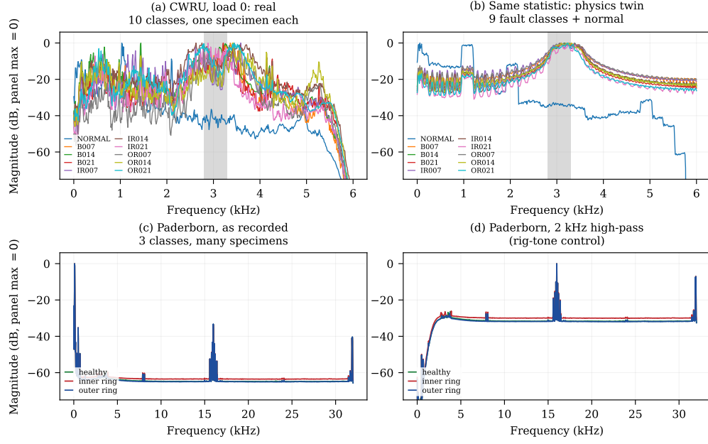
Figure 2: Class-mean magnitude spectra under the identical, unsmoothed statistic of Table 4. Each panel is normalized to its own maximum (0 dB); all four share the same -75 dB floor, the same linear frequency axis and the same per-class colours, and the shaded span marks the 2800–3300 Hz band whose energy fraction is quoted in Section 5. (a) CWRU, ten classes, one physical specimen each: visibly separated. (b) The physics twin, same statistic: the nine fault classes collapse into one band. Their median pairwise separation is 2.5 dB (minimum 0.9 dB), against 6.7 dB (minimum 3.7 dB) for the nine real classes, and across frequency the nine twin curves span a median of 6.5 dB against 18.8 dB. This is the whole negative result in one panel — the simulator produces nine faults whose mean spectra are interchangeable, so no classifier trained on them can carry the contrast that separates the real classes. (c) Paderborn as recorded: the 100 Hz rig line of Section 7 lands in the 93.75 Hz bin (with leakage into its neighbour at 109 Hz) and carries essentially all the energy, and the three damage classes are indistinguishable because everything else lies 60 dB below it. (d) The same recordings after a 2 kHz high-pass removes that line — the objection that one dominant tone is flattening the comparison. The 16 kHz rig resonance now dominates, yet the three class means still track each other to within a few dB across the whole band: the absence of class structure is not an artefact of the tone. Compare (d) with (a), where the same statistic separates the real classes by 10–30 dB.
