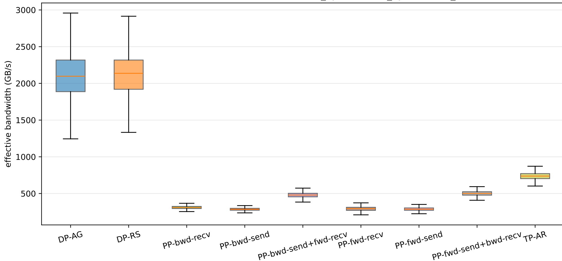
Per-event effective bandwidth — (\text{send\_bytes} + \text{recv\_bytes}) / \text{wall\_dur}
