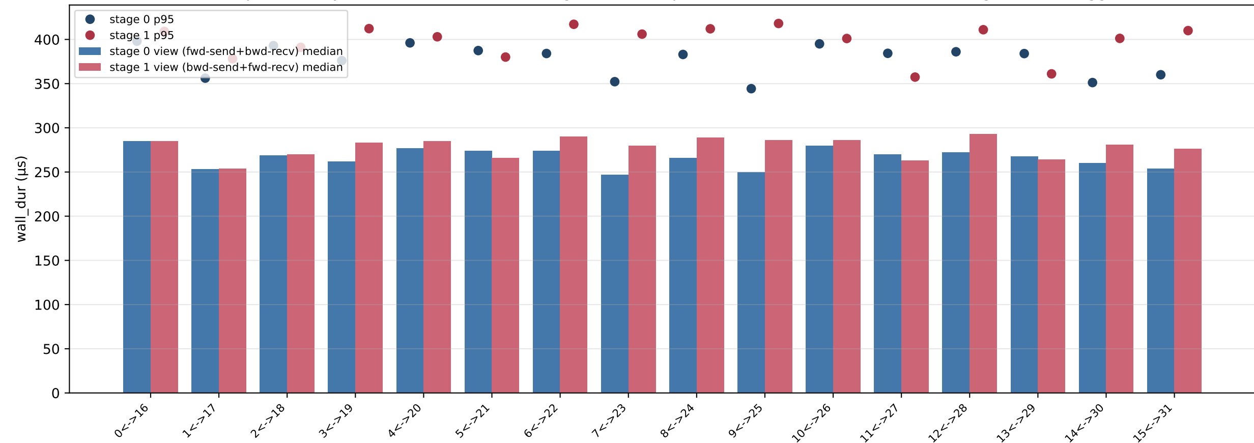
Per-PP-pair latency for the fused 1F1B exchange (both endpoints should see similar wait — divergence = straggler)
