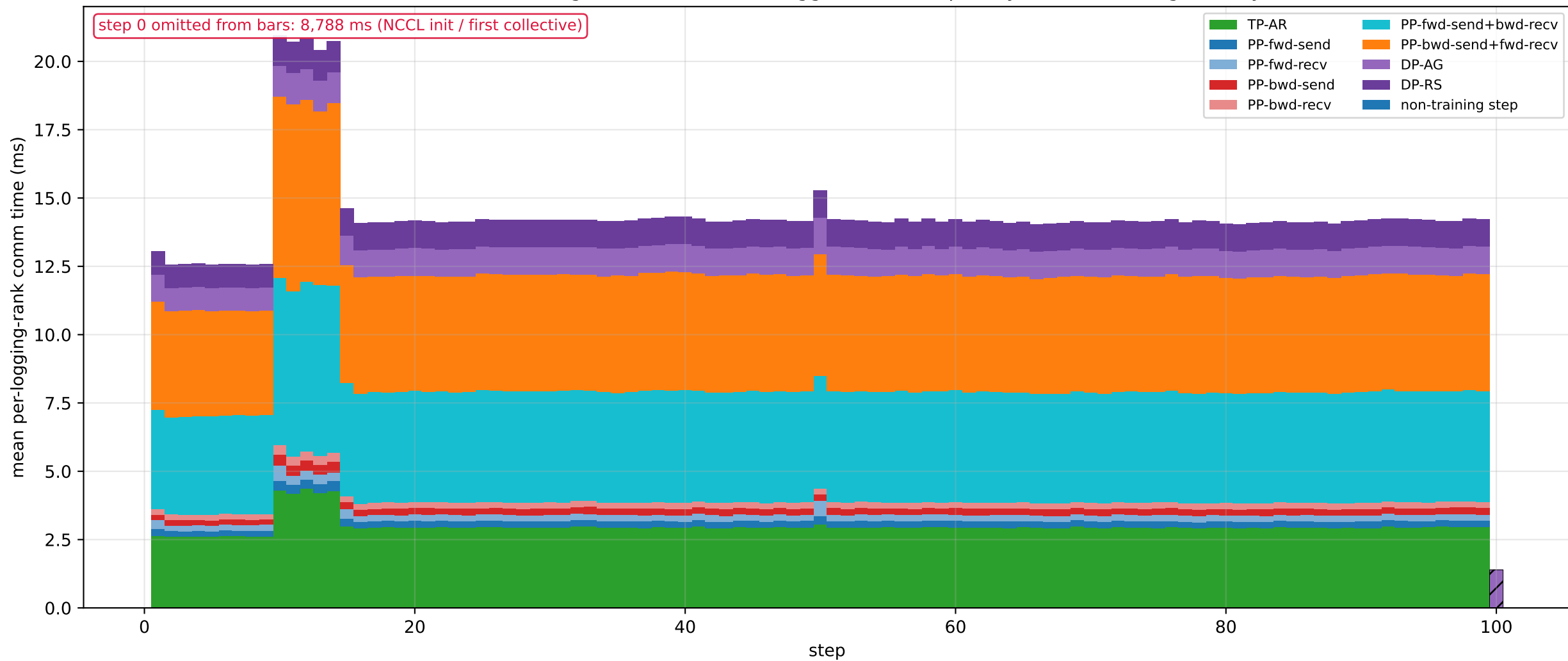
Per-step communication-time breakdown — TP + PP + DP (each event averaged over ranks that logged it; TP/DP per-layer traffic is stage-0 only)
