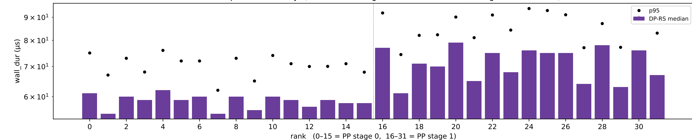
DP-RS — per-rank latency (n events on stage-0 ranks ~ 3200/rank, stage-1 ~ 100/rank)
