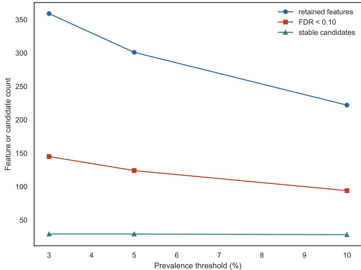
Filter threshold sensitivity
