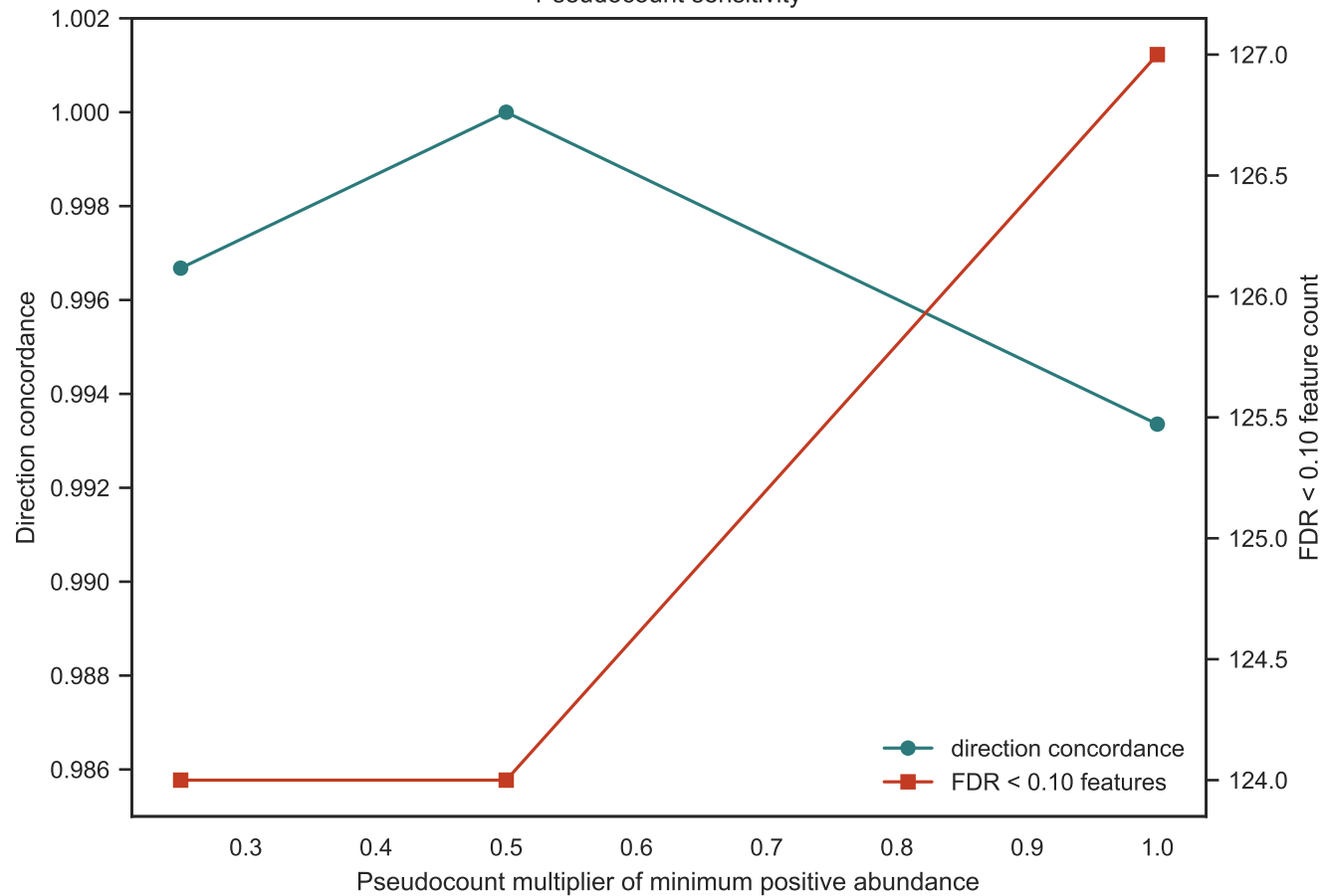
Pseudocount sensitivity
