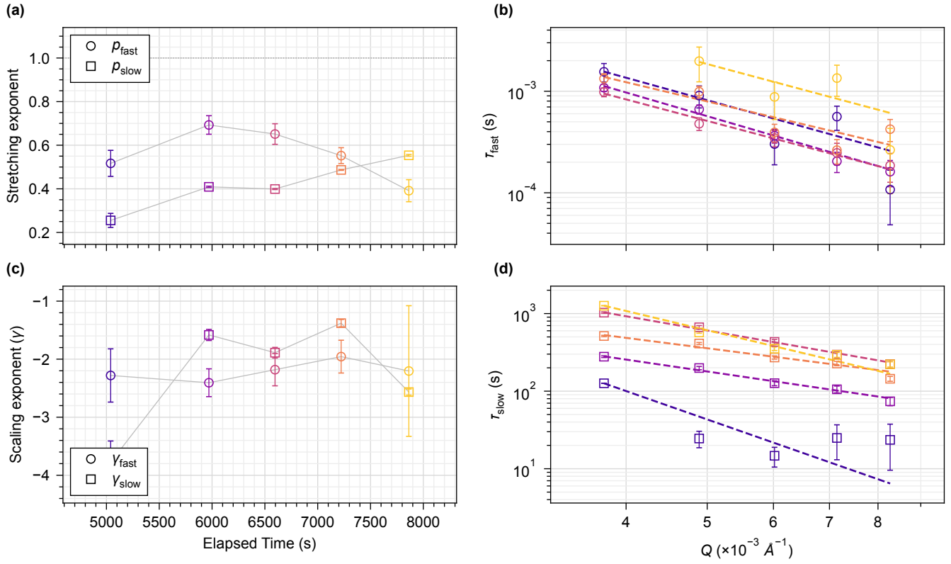
Figure S8: Additional parameters from global two-mode fits. Colors denote elapsed time as in Figure 3 of the main text (5040, 5970, 6596, 7222 and 7863 s, dark to light). (a) Stretching exponents shared across the five Q bins at each elapsed time. (b) Effective fast relaxation time versus Q . (c) Fitted scaling exponents \gamma_{\text{fast}} and \gamma_{\text{slow}} . (d) Effective slow relaxation time versus Q . Dashed lines in panels (b,d) are power-law fits \tau \propto Q^\gamma . At the final elapsed time the fast amplitude at the lowest Q bin has fallen to f = 0.012 \pm 0.004 and \tau_{\text{fast}} there is 1.1 \pm 1.3 s, three decades above every other bin and not measured; that point is omitted from (b) and from its power-law fit, which is why the final \gamma_{\text{fast}} has a larger uncertainty. The slow-mode quantities are extrapolations beyond the accessible delay range; \gamma_{\text{slow}} at the earliest elapsed time, -3.78 \pm 0.37 , lies well outside the -1.4 to -2.6 spanned by the other four, and is the least constrained of the set because the slow mode carries its smallest amplitude there. Grey lines connect points belonging to the same parameter and are guides to the eye; the dotted line in (a) marks p = 1 , the simple-exponential limit. Error bars are fit uncertainties.
