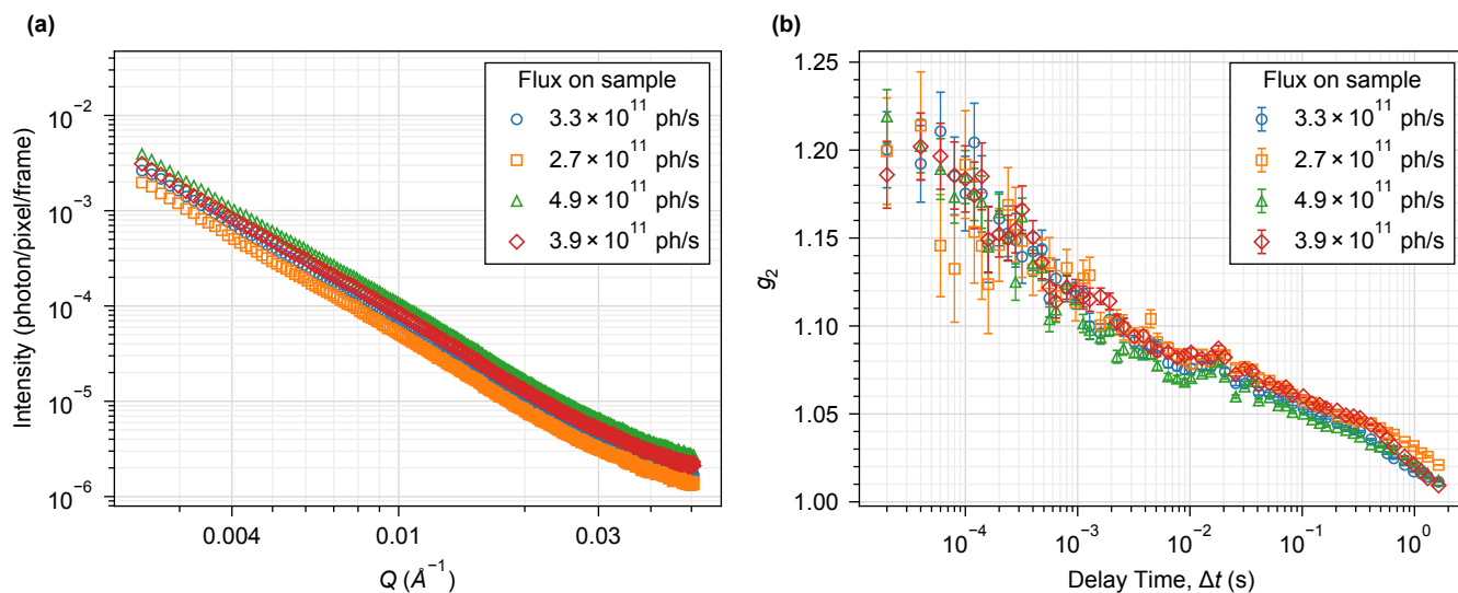
Figure S3: Flux-dependence control for SAXS and SA-XPCS. (a) SAXS profiles and (b) intensity autocorrelation functions from a 20 mg mL -1 (VPAVG) 30 sample at incident fluxes of 2.7 \times 10^{11} – 4.9 \times 10^{11} photons s -1 . The Q range shown in (a), 0.0024–0.051 Å -1 , covers the Q range of Figure 3a of the main text. Intensities in (a) are detector counts per pixel per frame, not on the absolute scale of Figure 3a. Panel (b) shows the lowest Q bin of this control configuration, Q = 0.00304 Å -1 ( 2\pi/Q \approx 206 nm). The legend orders the four conditions by nominal attenuator setting, which is not monotonic in flux. No systematic flux-dependent change is resolved over this range, which substantially exceeds the flux used in the main experiment.
