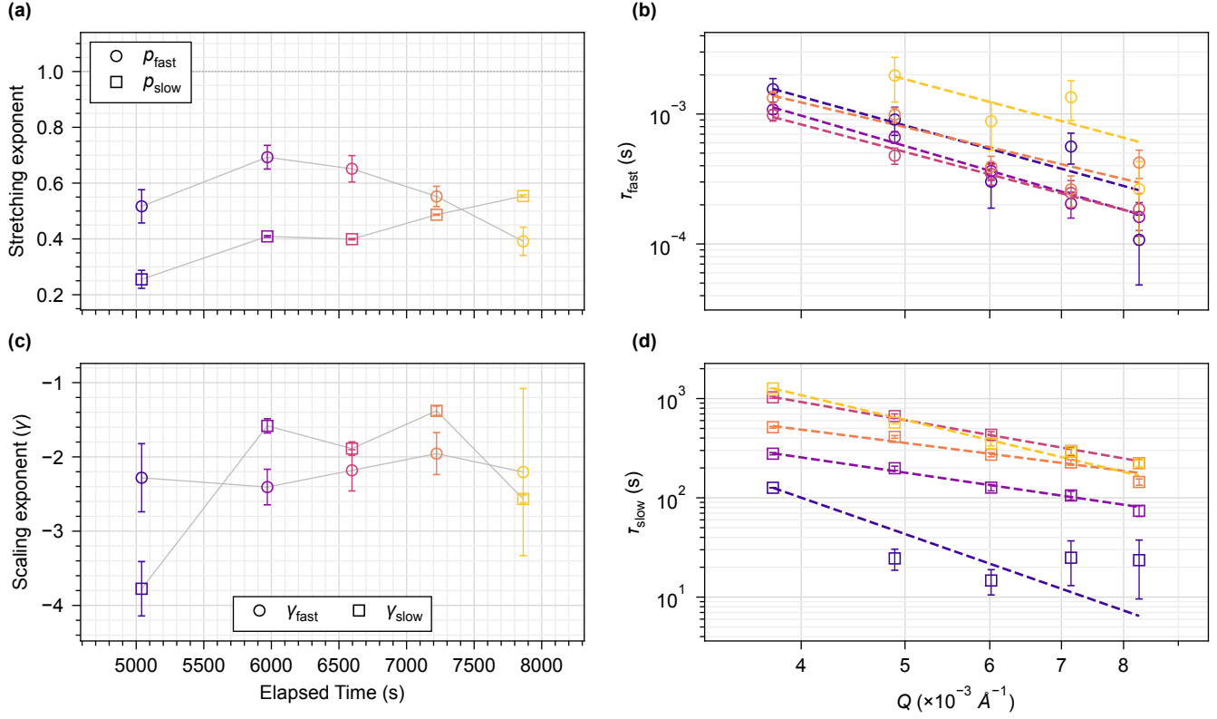
Figure S8: Additional parameters from global two-mode fits. Colors denote elapsed time as in Figure 3 of the main text (5040, 5970, 6596, 7222 and 7863 s, dark to light). (a) Stretching exponents shared across the five Q bins at each elapsed time. (b) Effective fast relaxation time versus Q . (c) Fitted scaling exponents \gamma_{\text{fast}} and \gamma_{\text{slow}} . (d) Effective slow relaxation time versus Q . Dashed lines in panels (b,d) are power-law fits \tau \propto Q^\gamma . At the final elapsed time the fast amplitude at the lowest Q bin has fallen to f = 0.012 \pm 0.004 and \tau_{\text{fast}} there is 1.1 \pm 1.3 s, three decades above every other bin and not measured; that point is omitted from (b) and from its power-law fit, which is why the final \gamma_{\text{fast}} has a larger uncertainty. The slow-mode quantities are extrapolations beyond the accessible delay range; \gamma_{\text{slow}} at the earliest elapsed time, -3.78 \pm 0.37 , lies well outside the -1.4 to -2.6 spanned by the other four, and is the least constrained of the set because the slow mode carries its smallest amplitude there. Grey lines connect points belonging to the same parameter and are guides to the eye; the dotted line in (a) marks p = 1 , the simple-exponential limit. Error bars are fit uncertainties.
