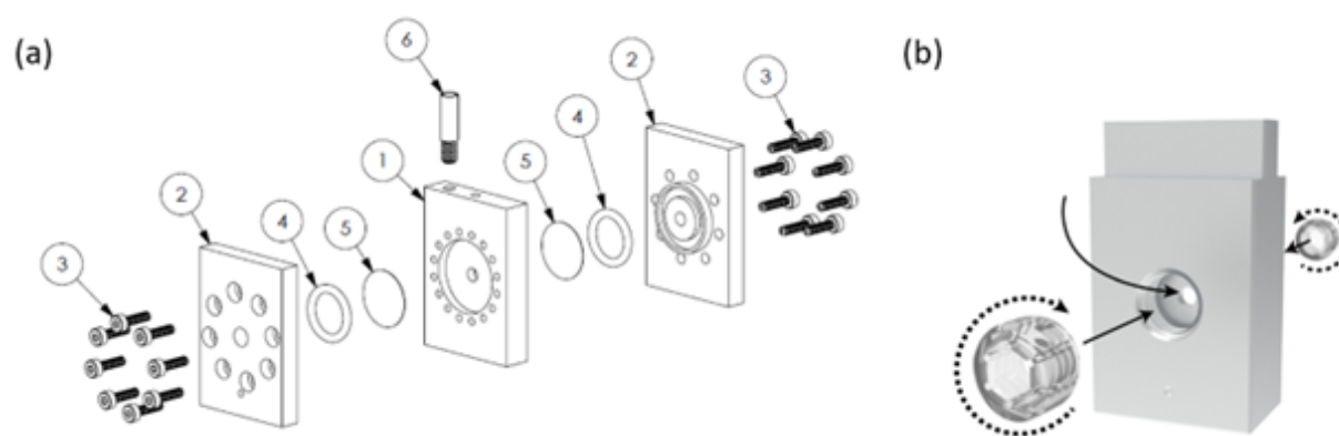
Figure S2: Sample cells used for liquid X-ray measurements. (a) Exploded view of the aluminum cell used for the 8-ID-I isothermal SA-XPCS experiment. The cylindrical chamber is 3 mm in diameter and 2 mm thick along the X-ray direction; 0.127 mm polycarbonate windows are compressed by Viton O-rings and bolted caps. During measurement, this cell was inserted into the anodized-aluminum holder of the Peltier-controlled stage described in Section 2.2; both the holder and cell were aluminum. (b) Screw-cap cell developed separately for automated handling; the dashed circles magnify the window seat. Only the bolted aluminum cell in panel (a) was used for measurements reported in the main text. The circled numerals in (a) identify the components: (1) the aluminum cell body, which contains the sample chamber; (2) the aluminum cap plates; (3) M2 screws, 8 mm long, which clamp the caps against the body; (4) Viton O-rings; (5) window disks cut from Kapton or polycarbonate sheet with a hammer-driven punch, polycarbonate being used for the measurements reported here; and (6) the handle used to withdraw the cell from the Quantum Northwest stage. Labels (2)–(5) appear on both sides of the body because the assembly is symmetric about the sample chamber.
