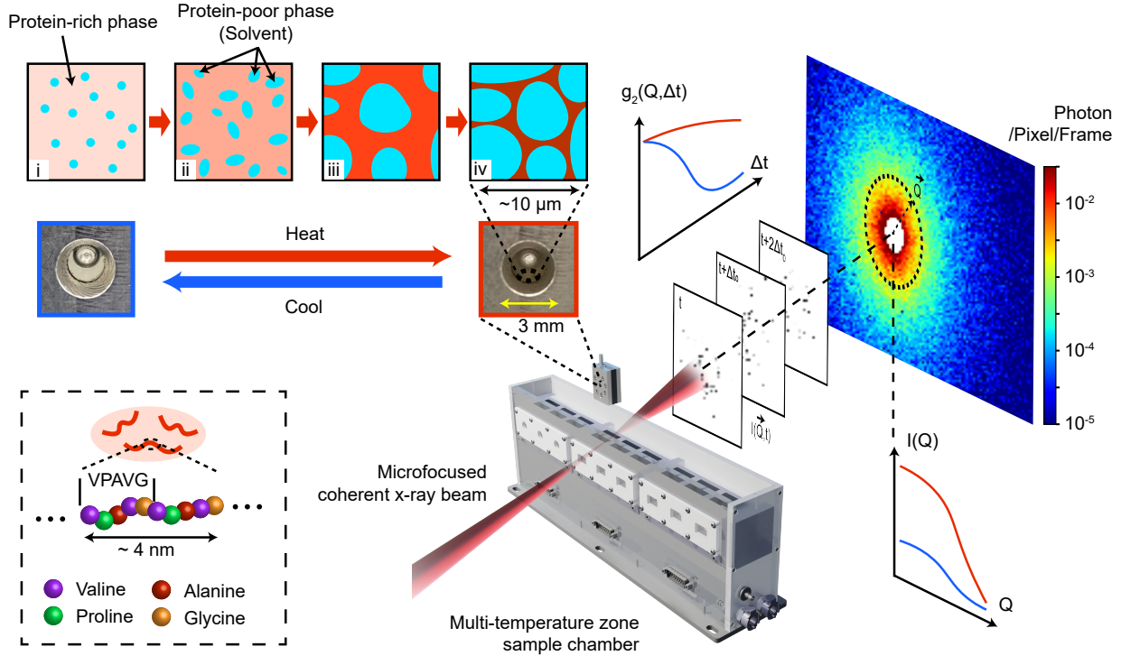
Figure 1: SA-XPCS measurement of thermally induced (\text{VPAVG})_{30} assembly at APS 8-ID-I. One set of sparse 20\ \mu\text{s} frames feeds two analyses. Averaging them gives the SAXS intensity I(Q) : how much structure the sample has at each length scale 2\pi/Q , which grows at low Q on heating. Correlating them in time gives g_2(Q, \Delta t) : how fast the structure at that same length scale rearranges, a decay meaning the density fluctuations at 2\pi/Q are still moving and a flat g_2 that they are frozen over the accessible delay. Both are sketched beside the detector (red: assembled; blue: dispersed; illustrative, not data). Center: the aluminum cell, liquid chamber 3mm across, below and above the transition. Lower left: one (\text{VPAVG})_{30} repeat, residues colored as keyed. Right: the frame-averaged detector image, color bar in photons per pixel per frame, white center the beamstop mask; the graininess is sparse counting statistics, not resolved speckle. Upper left, stages i-iv: a conceptual illustration, not a real-space observation, of the candidate viscoelastic phase-separation pathway, 20,27 in which protein-poor solvent pools (cyan) nucleate and grow within the still-continuous protein-rich phase (deepening red: more protein), coarsening it toward a network-like morphology.
