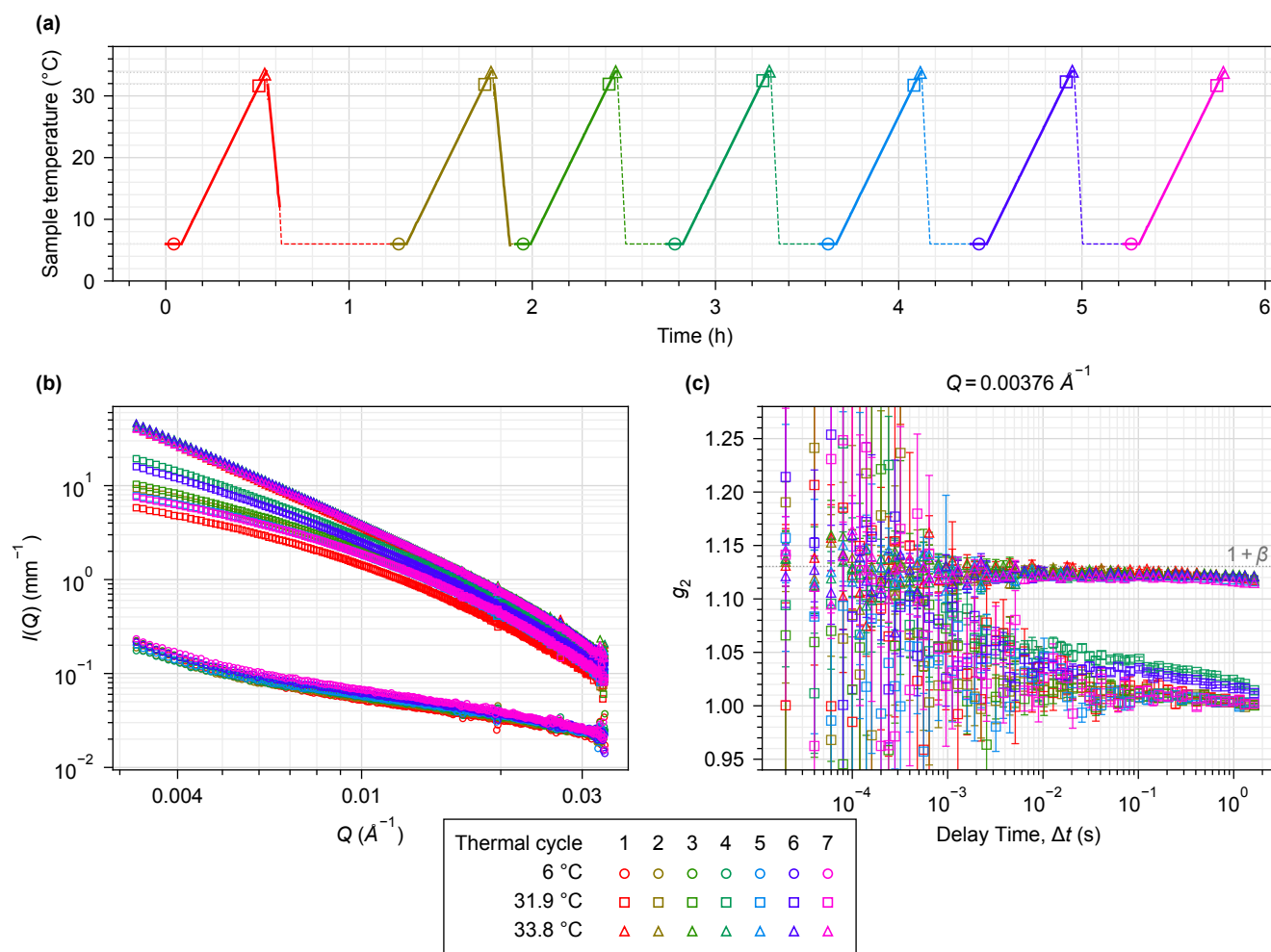
Figure S5: Thermal-cycling repeatability of the SA-XPCS sample: one aliquot—a separate loading from the isothermal experiment of Figure 3 of the main text—through seven consecutive cycles. (a) Sample temperature over the 5.8 h sequence. Solid curves are measured: the stage RTD was read once per 2 s acquisition. No acquisitions were taken while the sample cooled, so no temperature was recorded over those intervals; the dashed curves there are not data but the profile projected from the control protocol, which was fixed at 10^\circ\text{C min}^{-1} cooling until 6^\circ\text{C} followed by a hold at 6^\circ\text{C} until the next ramp. Open symbols mark, at the time and temperature at which it was taken, every acquisition group that is plotted in (b) and (c), so each lower-panel curve can be traced to its point in the thermal history. (b) Buffer-subtracted SAXS on an absolute scale at 6^\circ\text{C} (circles, 32–41 surviving acquisitions averaged; see Section 7.2), 31.9^\circ\text{C} (squares, acquisitions 241–250) and 33.8^\circ\text{C} (triangles, acquisitions 261–270). Each group is placed on the absolute scale with the mean ion-chamber readings of the acquisitions it contains, and the averaged buffer (69 surviving of 89 acquisitions, D0077 and D0080) is subtracted with no empirical scale factor, exactly as in Figure 3a. (c) Correlation functions at the lowest Q bin for the two high-temperature states; the dotted line is 1 + \beta with \beta the contrast measured in Figure S8. Error bars are the measured pointwise g_2 uncertainties; the y axis is capped so that a few short-delay caps clip. One key serves all three panels: its columns are the seven thermal cycles, numbered along the top and colored on the same scale Figure 3 of the main text uses for elapsed time, and its rows are the three temperature states, labeled at the left and distinguished by marker shape.
