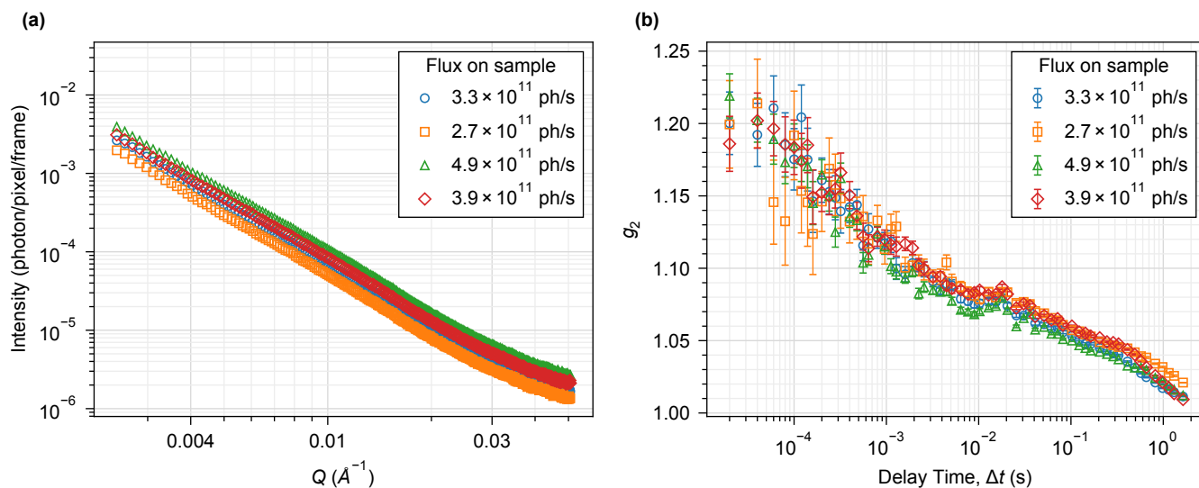
Figure S3: Flux-dependence control for SAXS and SA-XPCS. (a) SAXS profiles and (b) intensity autocorrelation functions from a 20 \text{ mg mL}^{-1} (VPAVG) 30 sample at incident fluxes of 2.7 \times 10^{11} – 4.9 \times 10^{11} \text{ photons s}^{-1} . The Q range shown in (a), 0.0024 – 0.051 \text{ \AA}^{-1} , covers the Q range of Figure 3a of the main text. Intensities in (a) are detector counts per pixel per frame, not on the absolute scale of Figure 3a. Panel (b) shows the lowest Q bin of this control configuration, Q = 0.00304 \text{ \AA}^{-1} ( 2\pi/Q \approx 206 \text{ nm} ). The legend orders the four conditions by nominal attenuator setting, which is not monotonic in flux. No systematic flux-dependent change is resolved over this range, which substantially exceeds the flux used in the main experiment.
