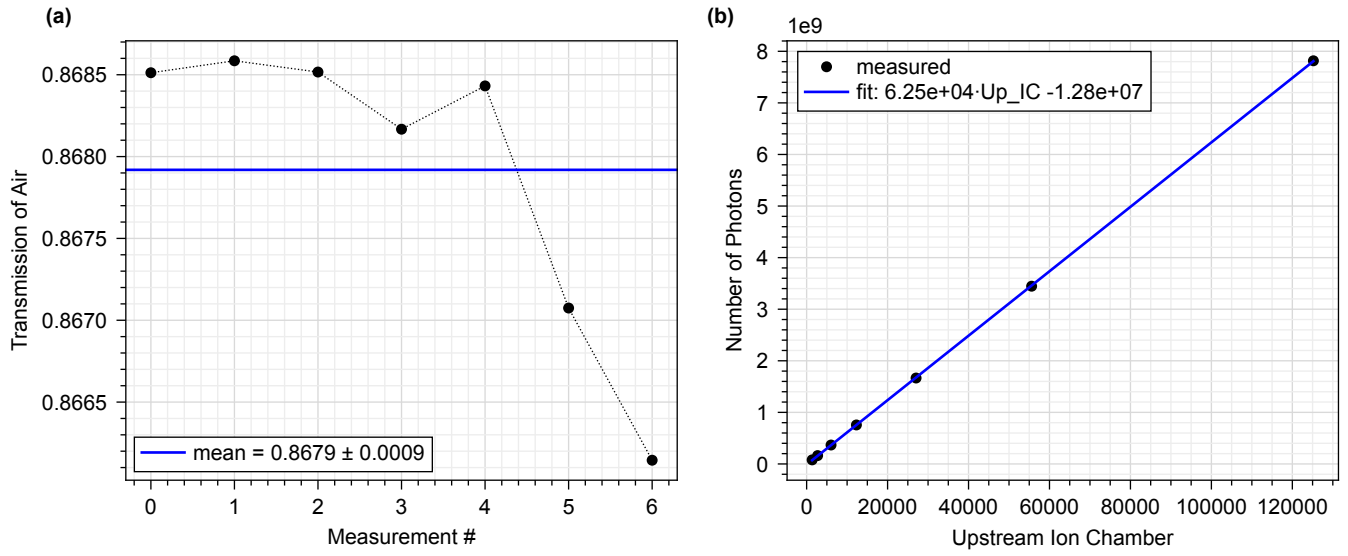
Figure S7: Transmission and photon-flux calibration for conversion to absolute scattering cross section. (a) Air-path transmission across seven measurements in the attenuation series; the line marks the mean, 0.8679 \pm 0.0009 (standard deviation). (b) Photon counts recorded by a calibrated PIN diode as a function of the upstream ion-chamber readout (both in the scaled detector units of the calibration series); the line is the linear calibration fit, from which the incident flux follows as F = (A \cdot \text{Up\_IC})/t_{\text{exp}} + B .
