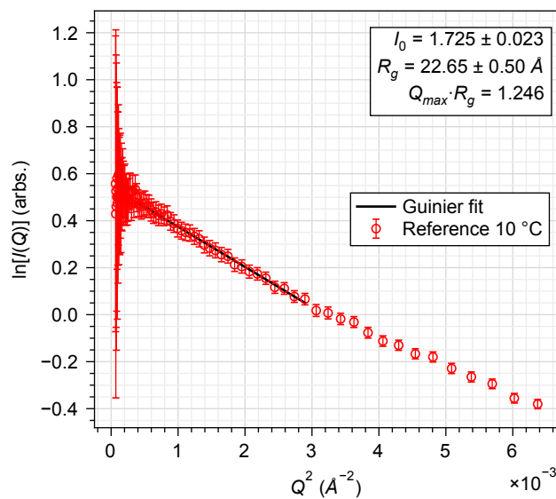
Figure S4: Guinier analysis of the Reference aliquot at 10 °C. Weighted linear fit of \ln I(Q) against Q^2 over 0.020 \leq Q \leq 0.055 \text{ \AA}^{-1} (so Q_{\max} R_g = 1.246 ), giving an apparent R_g = 22.65 \pm 0.50 \text{ \AA} and I_0 = 1.725 \pm 0.023 in the arbitrary intensity units of the reduced 12-ID-B profiles. Points are plotted over the wider range 0.005 \leq Q \leq 0.080 \text{ \AA}^{-1} for context; error bars are the propagated intensity uncertainties, \sigma_I/I .
