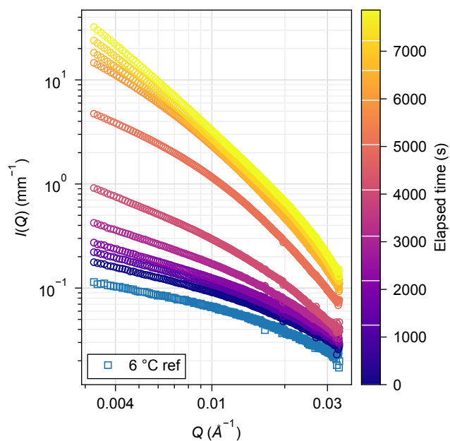
Figure S6: Complete isothermal SAXS evolution of (VPAVG) 30 at 30 °C, buffer-subtracted and on the same absolute scale as Figure 3a of the main text, using the same buffer measurement. The 6 °C reference and profile at the start of the hold are followed by profiles from 1249 to 7863 s. White marks on the color bar give the elapsed time of each measured profile. Colors here are scaled linearly over the full 0–7863 s range and therefore do not match the discrete colors used for the same times in Figure 3; read times from the color bar. The subset from 5039 to 7863 s corresponds to the SAXS and SA-XPCS data analyzed in Figure 3 of the main text.
