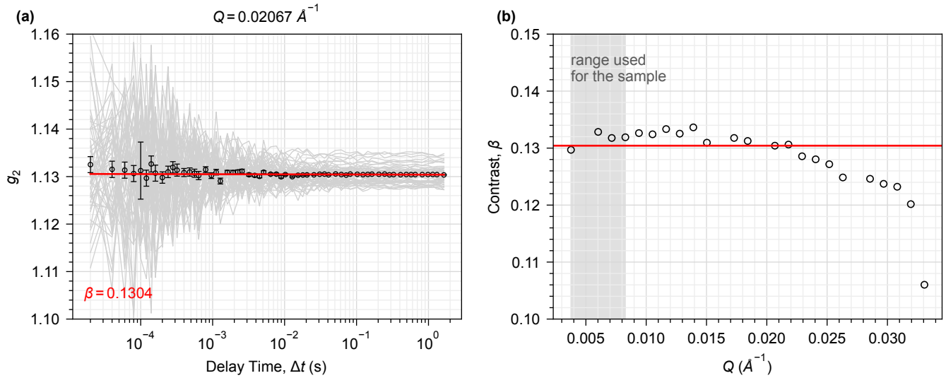
Figure S8: Measurement of the instrumental speckle contrast \beta on a static reference. (a) Correlation functions of a 10 nm nano-porous glass standard at Q = 0.02067 \text{ \AA}^{-1} , the best-counted bin whose averaged correlation function is flat to within its uncertainties: 50 individual repeat acquisitions (grey) and their average (black, with the measured pointwise uncertainties). The red line is a straight-line fit in \log \Delta t ; it is flat to 1.7 standard deviations with reduced \chi^2 = 1.02 , as a static sample requires, and its level gives \beta = 0.13042 \pm 0.00001 . (b) The same procedure applied bin by bin. \beta is essentially independent of Q across the shaded range used for the sample; the red line is the fixed value from (a). Above Q \approx 0.021 \text{ \AA}^{-1} , outside that range, \beta falls off as the finite longitudinal coherence length set by the Si(111) monochromator begins to limit the contrast. Four of the five bins used for the sample return \beta = 0.1297, 0.1328, 0.1318 and 0.1319 , all within 2% of it. Four bins out of 27 whose averaged correlation function is not flat (reduced \chi^2 > 5 , detector and parasitic-scattering artifacts) are omitted, one of them at Q = 0.00489 \text{ \AA}^{-1} inside the shaded range.
