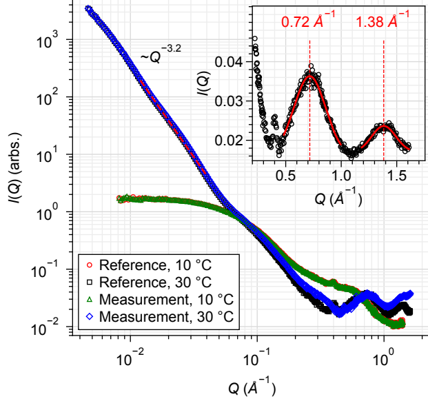
Figure 2: Temperature-dependent structure and reversibility of (\text{VPAVG})_{30} . At 10^\circ\text{C} , the Measurement and Reference profiles overlap and the Reference data give an apparent R_g = 22.65 \pm 0.50 \text{ \AA} (Figure S3). Heating produces an approximate Q^{-3.2} low- Q response and peaks at Q = 1.38 and 0.72 \text{ \AA}^{-1} , corresponding to real-space spacings of approximately 4.5 and 8.8 \text{ \AA} , respectively. The dashed line is an unweighted power-law fit to the Reference profile at 30^\circ\text{C} over 0.012 < Q < 0.040 \text{ \AA}^{-1} . Inset: the high- Q region of that same profile (open circles, same arbitrary intensity units as the main panel); red curves are independent Gaussian-plus-linear-background fits over 0.48 < Q < 1.00 and 1.18 < Q < 1.70 \text{ \AA}^{-1} , and the red dashed lines and labels mark the fitted peak centers. The recovery and reproducible re-formation of these signatures demonstrate a thermally reversible structural transition within experimental sensitivity.
