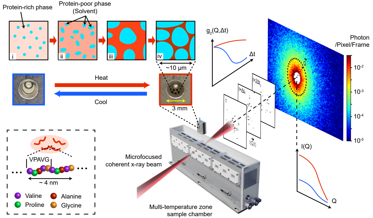
Figure 1: SA-XPCS measurement of thermally induced (VPAVG) 30 assembly at APS 8-ID-I. One set of sparse 20 μs frames feeds two analyses. Averaging them gives the SAXS intensity I(Q) : how much structure the sample has at each length scale 2\pi/Q , which grows at low Q on heating. Correlating them in time gives g_2(Q, \Delta t) : how fast the structure at that same length scale rearranges, a decay meaning the density fluctuations at 2\pi/Q are still moving and a flat g_2 that they are frozen over the accessible delay. Both are sketched beside the detector (red: assembled; blue: dispersed; illustrative, not data). Center: the aluminum cell, liquid chamber 3mm across, below and above the transition. Lower left: one (VPAVG) 30 repeat, residues colored as keyed. Right: the frame-averaged detector image, color bar in photons per pixel per frame, white center the beamstop mask; the graininess is sparse counting statistics, not resolved speckle. Upper left, stages i-iv: a conceptual illustration, not a real-space observation, of the candidate viscoelastic phase-separation pathway, 20,27 in which protein-poor solvent pools (cyan) nucleate and grow within the still-continuous protein-rich phase (deepening red: more protein), coarsening it toward a network-like morphology.
