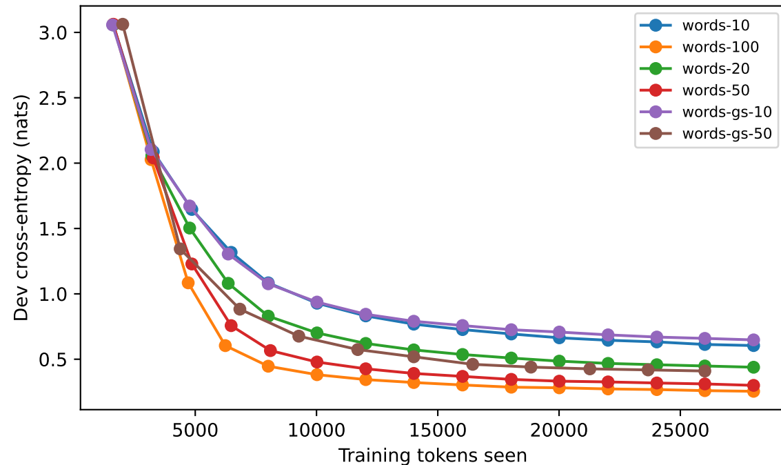
Dev Cross Entropy with different lexicons (d=8)
