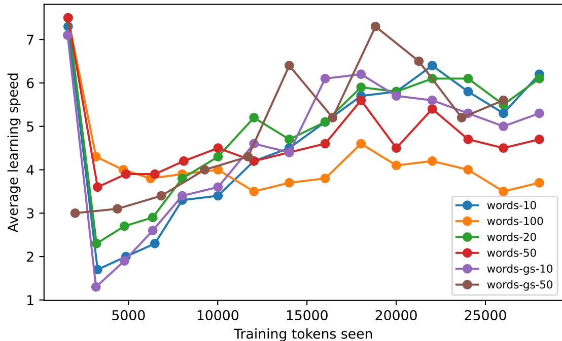
Learning speed with different lexicons (d=8)
