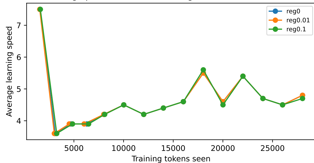
Learning speed with different Regularization (0, 0.01, 0.1)
