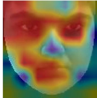
Pyramid Attention
