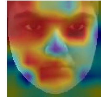
Pyramid Attention
