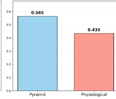
Influence Factors
