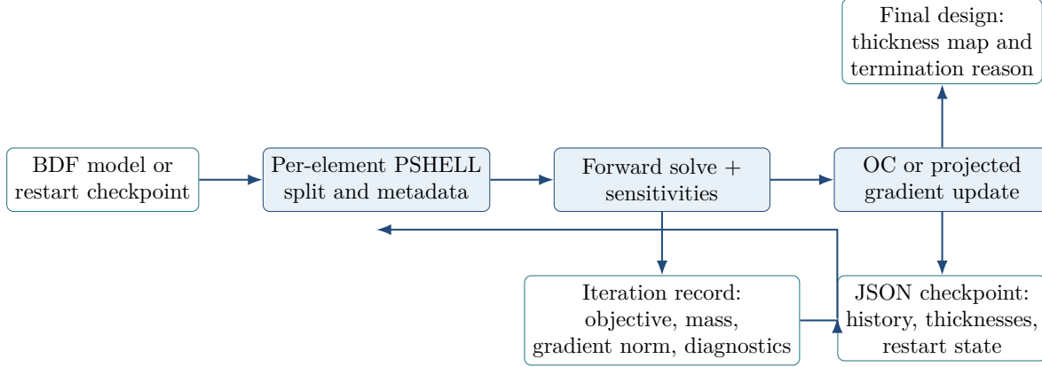
Figure 5: Optimization workflow now implemented in the repository. Shell thicknesses and, in the generalized sizing path, bar areas are created through per-element property splitting; each iteration records objective and solver-health data, and the process can be checkpointed and restarted from JSON.
