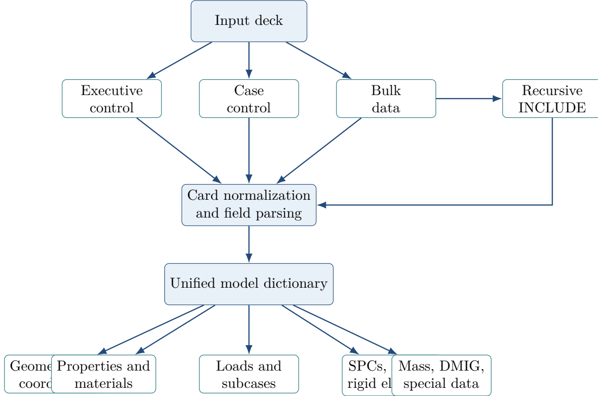
Figure 2: Conceptual view of the accepted input structure. The parser resolves INCLUDE chains, extracts case-control directives, and then builds a unified internal model from the bulk-data cards.
