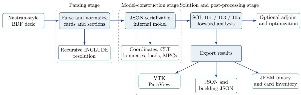
Figure 1: Repository-level software architecture. The checked-in implementation is organized as parse, solve, and export stages, with optional adjoint and optimization hooks attached after the forward solution.
