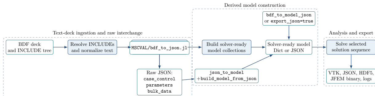
Figure 6: Detailed workflow from a Nastran-style BDF deck to raw JSON, the derived solver-ready model, and the final solution/export stages. The raw JSON bridge is intentionally placed before the code computes derived material, laminate, coordinate, and constraint data.
