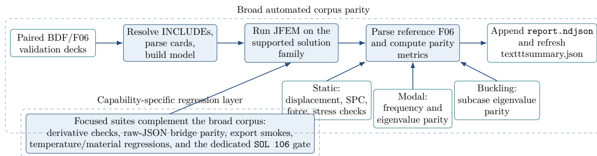
Figure 8: Validation workflow used by the repository. Broad automated corpus parity is recorded deck-by-deck in NDJSON and summarized in JSON, while focused regression suites guard specific capabilities that a broad corpus snapshot may miss or under-sample.
