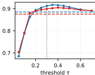
Accuracy (higher is better)
