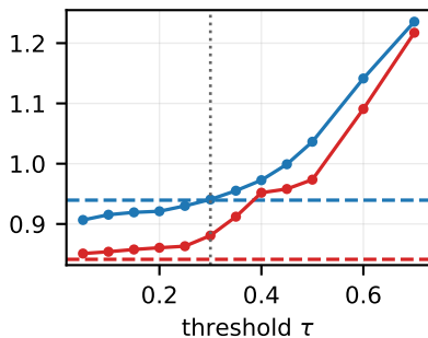
RMSE (lower is better)
