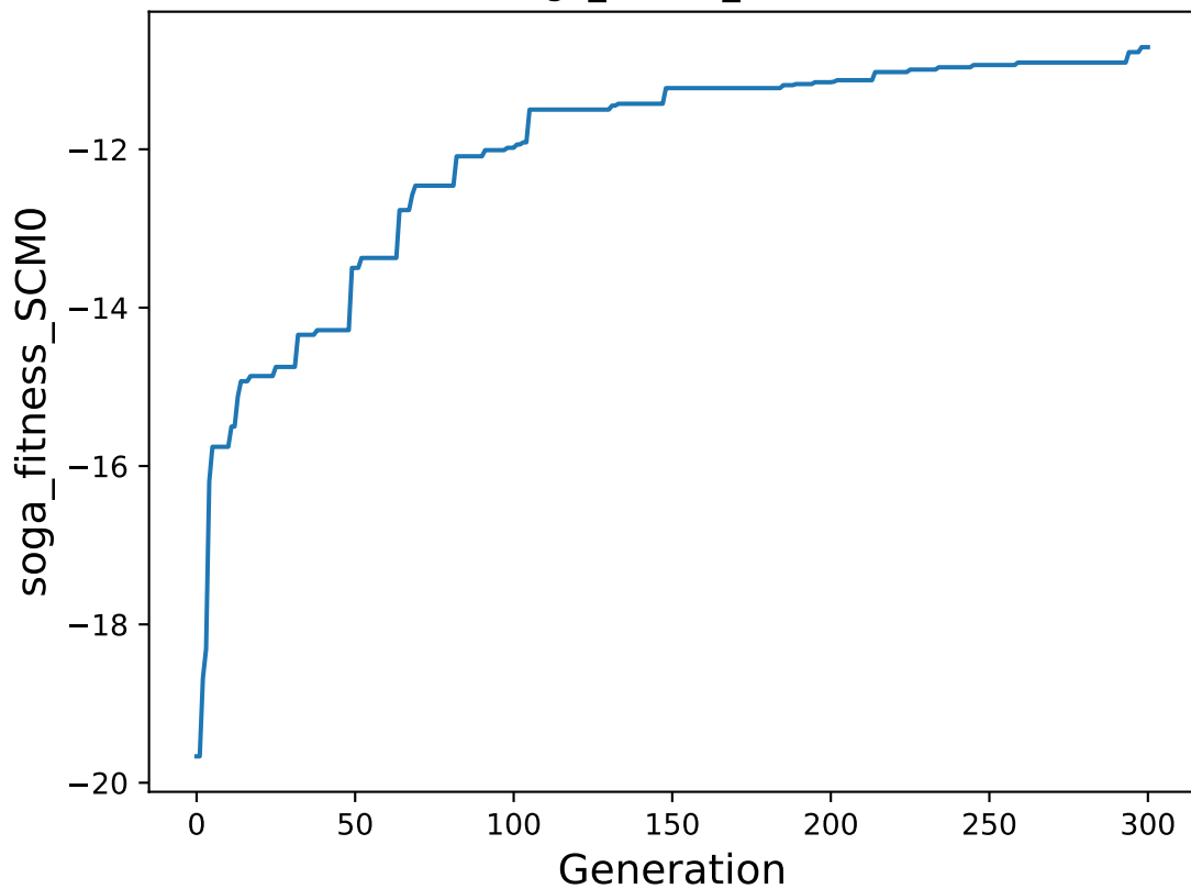
soga_fitness_SCM0
