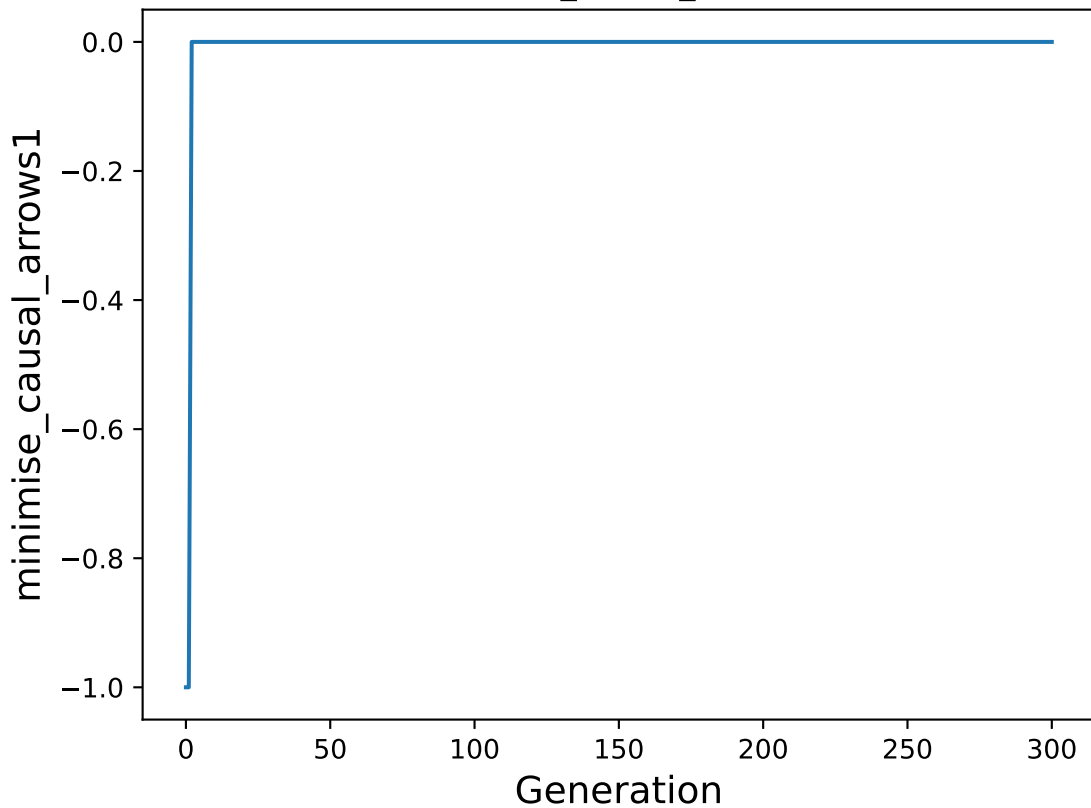
minimise_causal_arrows1
