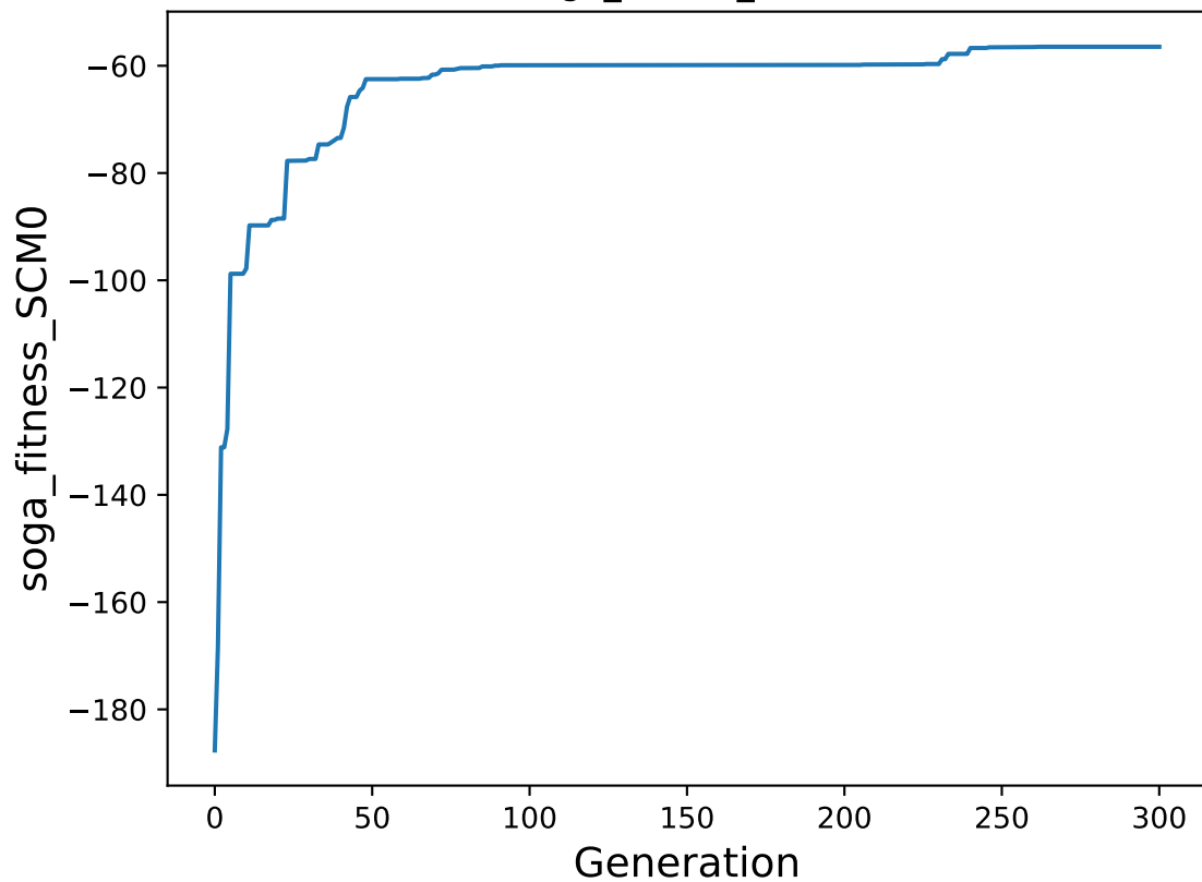
soga_fitness_SCM0
