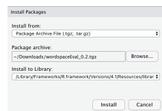
wordspaceEval
