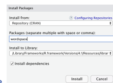
wordspace
