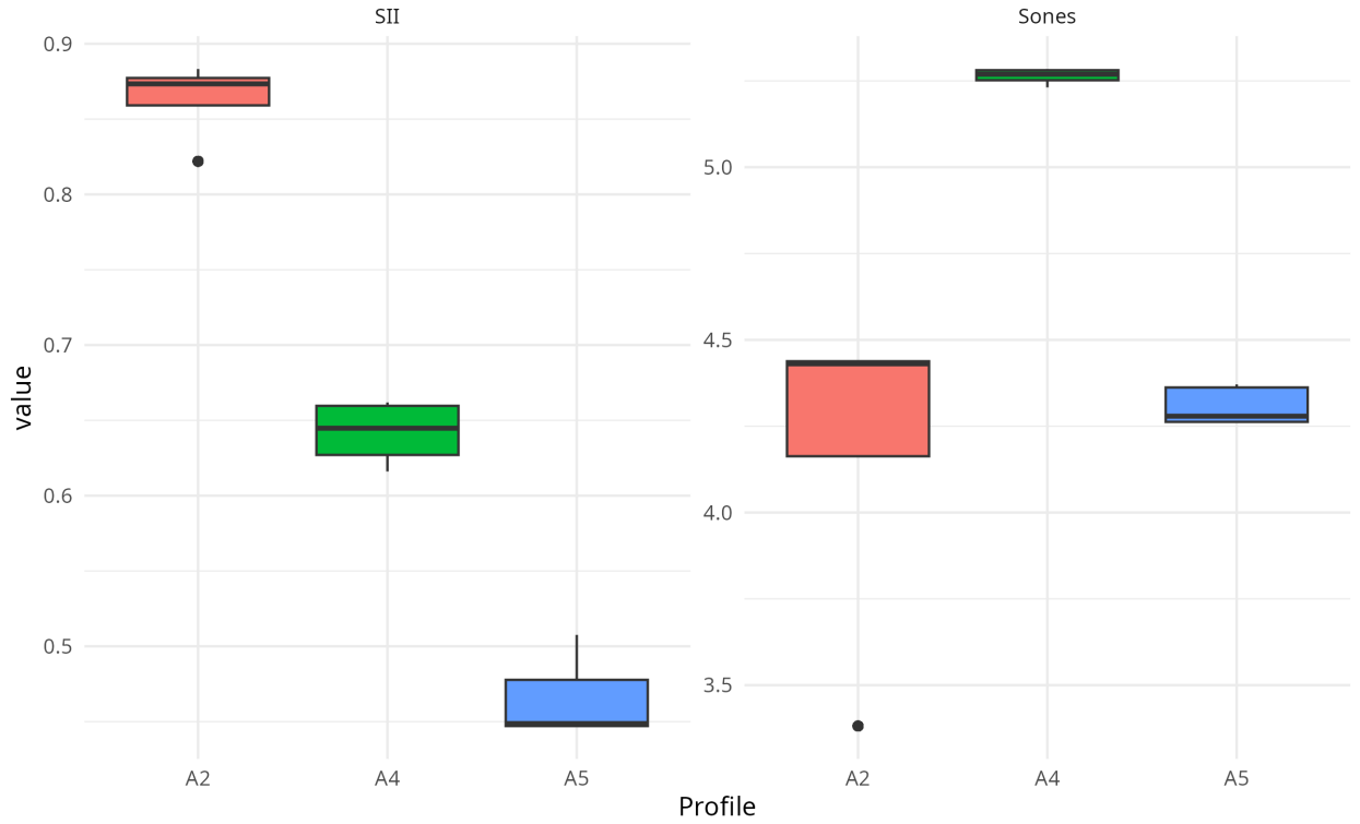
Figure 4. Distribution of resulting ANSI SII scores and physiological loudness penalties across 768 permutations ( 256 \times 3 profiles) for clinical profiles A2 (Reverse Slope), A4 (Profound), and A5 (Severe), illustrating high heuristic parameter sensitivity.
