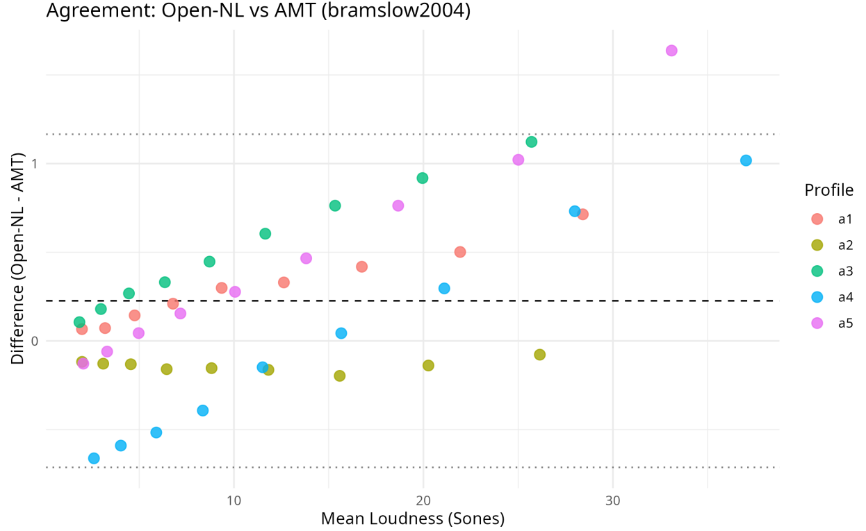
491 Figure 2. Difference plot demonstrating excellent approximate convergence between Open-NL's 492 stationary spectral C++ engine and AMT's dynamic time-domain simulation (bramslow2004) 493 across 45 canonical evaluation points.
