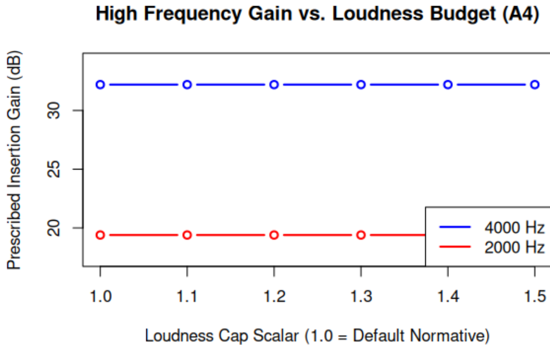
427 Figure 6. High-Frequency Gain vs. Loudness Budget Cap for Profile A4 (65 dB SPL).
