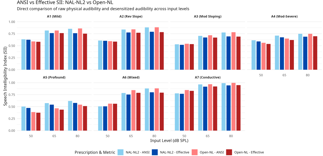
Figure 1: Comparison of ANSI SII (Raw Physical Audibility) vs Desensitized SII for NAL-NL2 and Open-NL across 50, 65, and 80 dB SPL Inputs.
