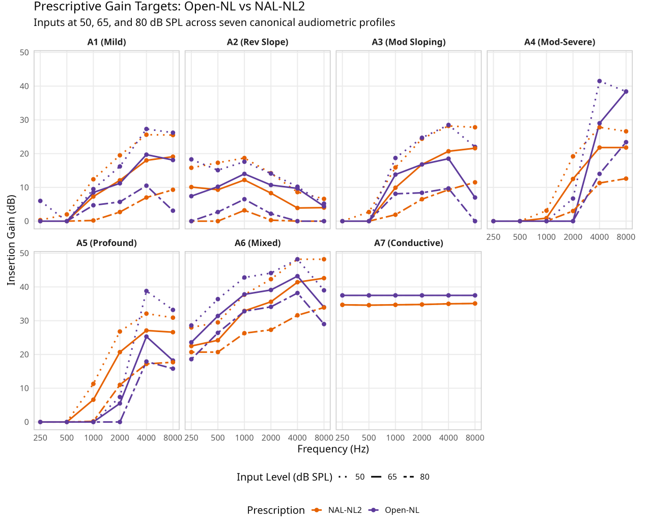
Figure 4. Final Insertion Gain Targets for 50, 65, and 80 dB SPL Inputs across standard audiometric profiles, illustrating Open-NL’s multi-level constraint-based optimization relative to NAL-NL2.
