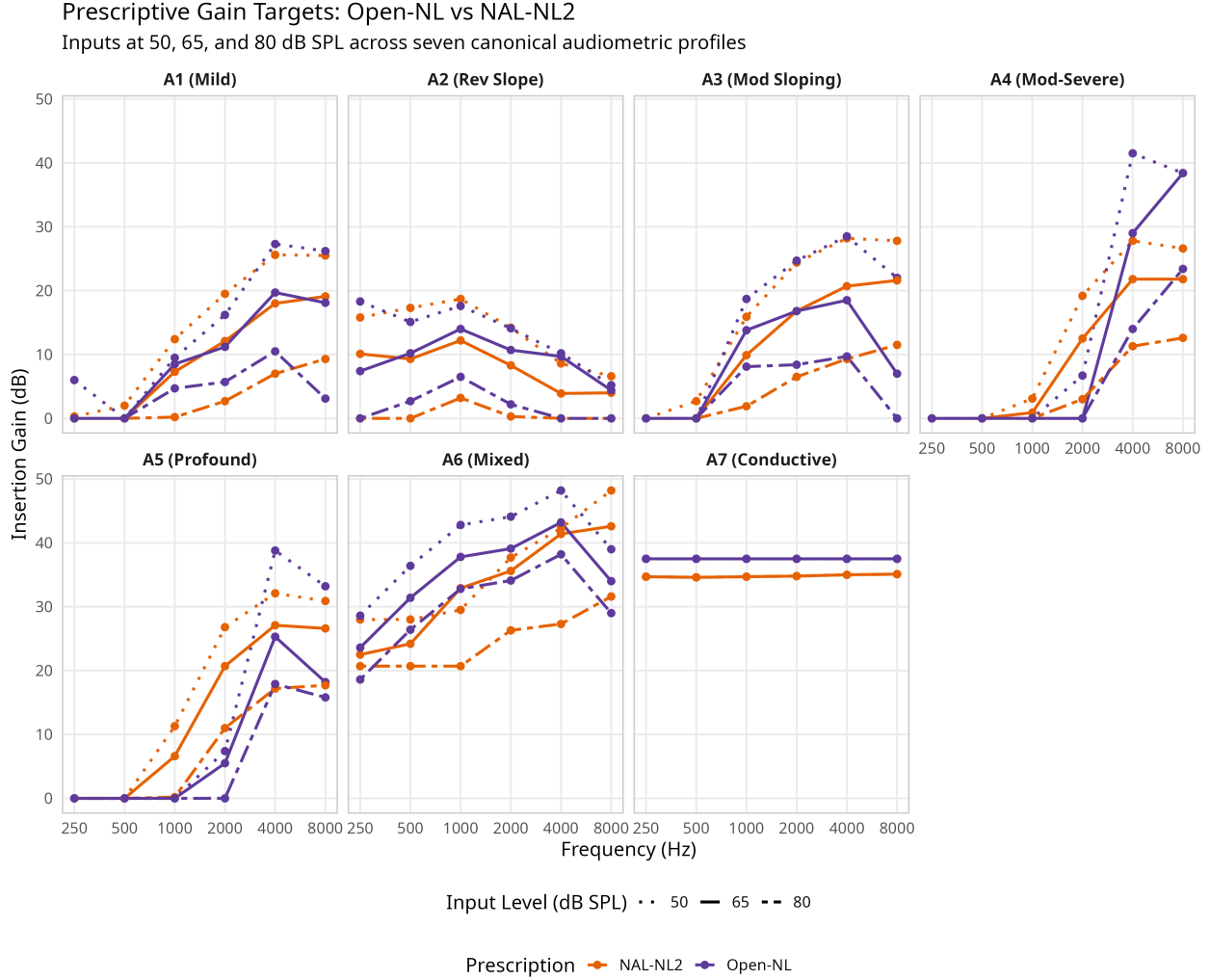
Figure 2: Final Insertion Gain Targets for 50, 65, and 80 dB SPL Inputs across standard audiometric profiles, illustrating Open-NL’s multi-level constraint-based optimization relative to NAL-NL2.
