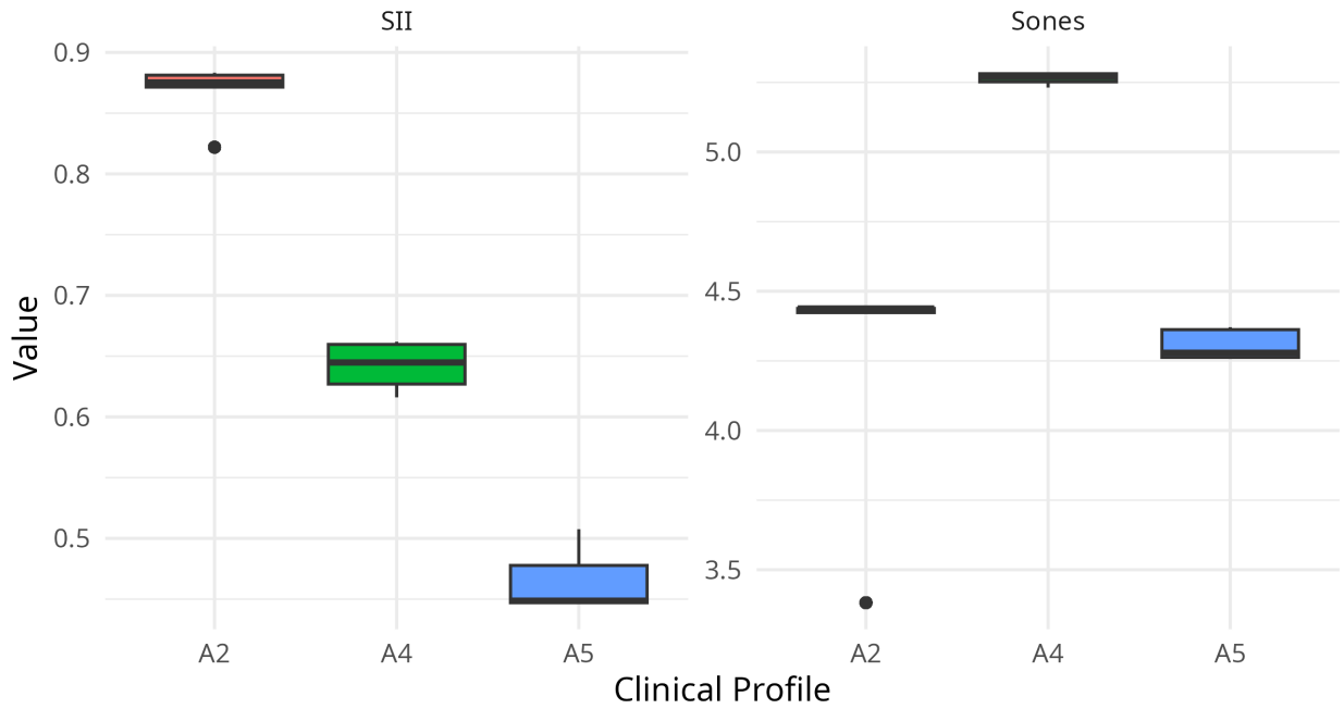
637 Figure 4. Distribution of maximized ANSI SII scores and physiological loudness penalties 638 across 768 extreme hyperparameter permutations for clinical profiles A2 (Reverse Slope), A4 639 (Profound), and A5 (Severe).
