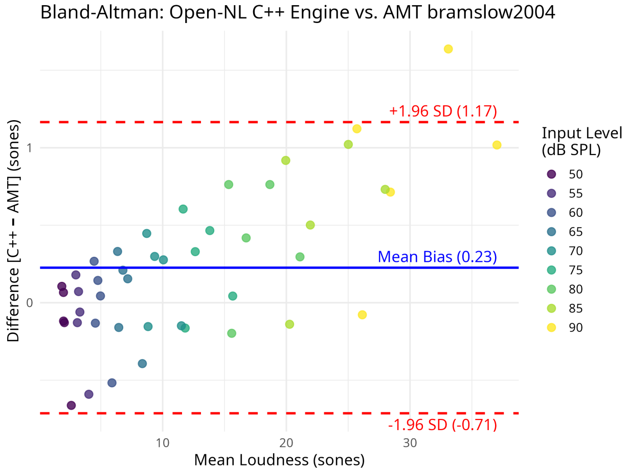
Figure 2. Bland-Altman difference plot between Open-NL’s stationary spectral C++ engine and AMT’s dynamic time-domain simulation ( bramslow2004 ) across 45 evaluation points. The solid blue line indicates mean bias (+0.23 sones), and dashed red lines indicate 95% Limits of Agreement [-0.71, +1.17].
