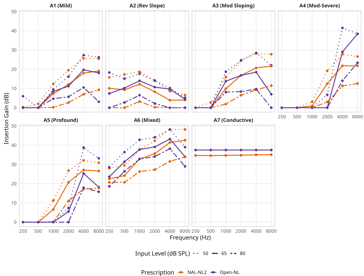
Figure 2: Final Insertion Gain Targets for 50, 65, and 80 dB SPL Inputs across standard audiometric profiles, illustrating Open-NL's multi-level constraint-based optimization relative to NAL-NL2.
