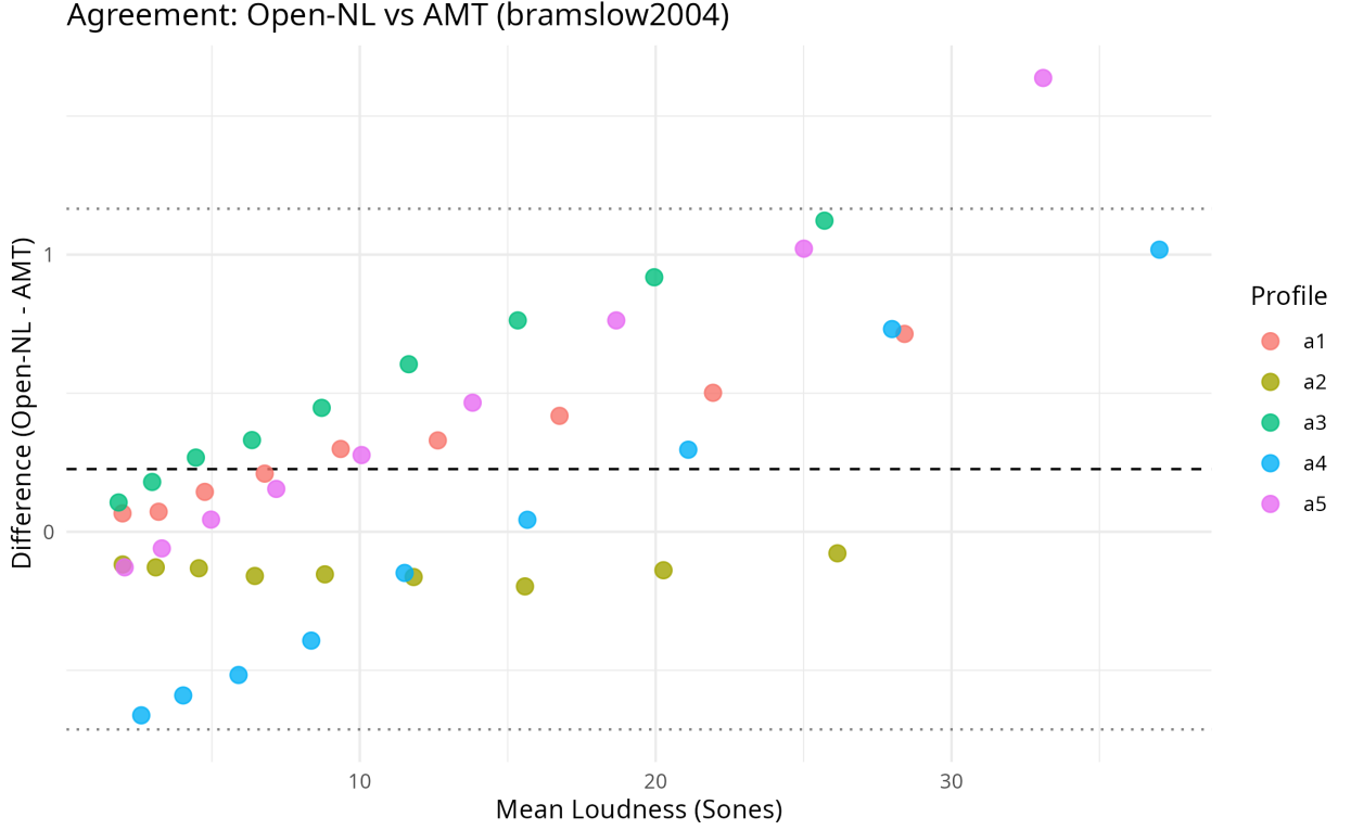
475 Figure 2. Difference plot demonstrating excellent approximate convergence between Open-NL's 476 stationary spectral C++ engine and AMT's dynamic time-domain simulation (bramslow2004) 477 across 45 canonical evaluation points.
