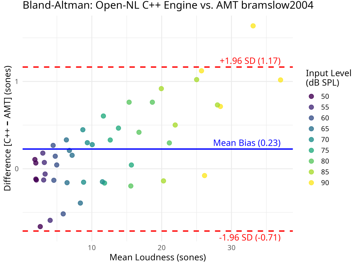
468 Figure 2. Bland-Altman difference plot between Open-NL's stationary spectral C++ engine 469 and AMT's dynamic time-domain simulation ( bramslow2004 ) across 45 evaluation points. 470 The solid blue line indicates mean bias (+0.23 sones), and dashed red lines indicate 95% 471 Limits of Agreement [-0.71, +1.17].
