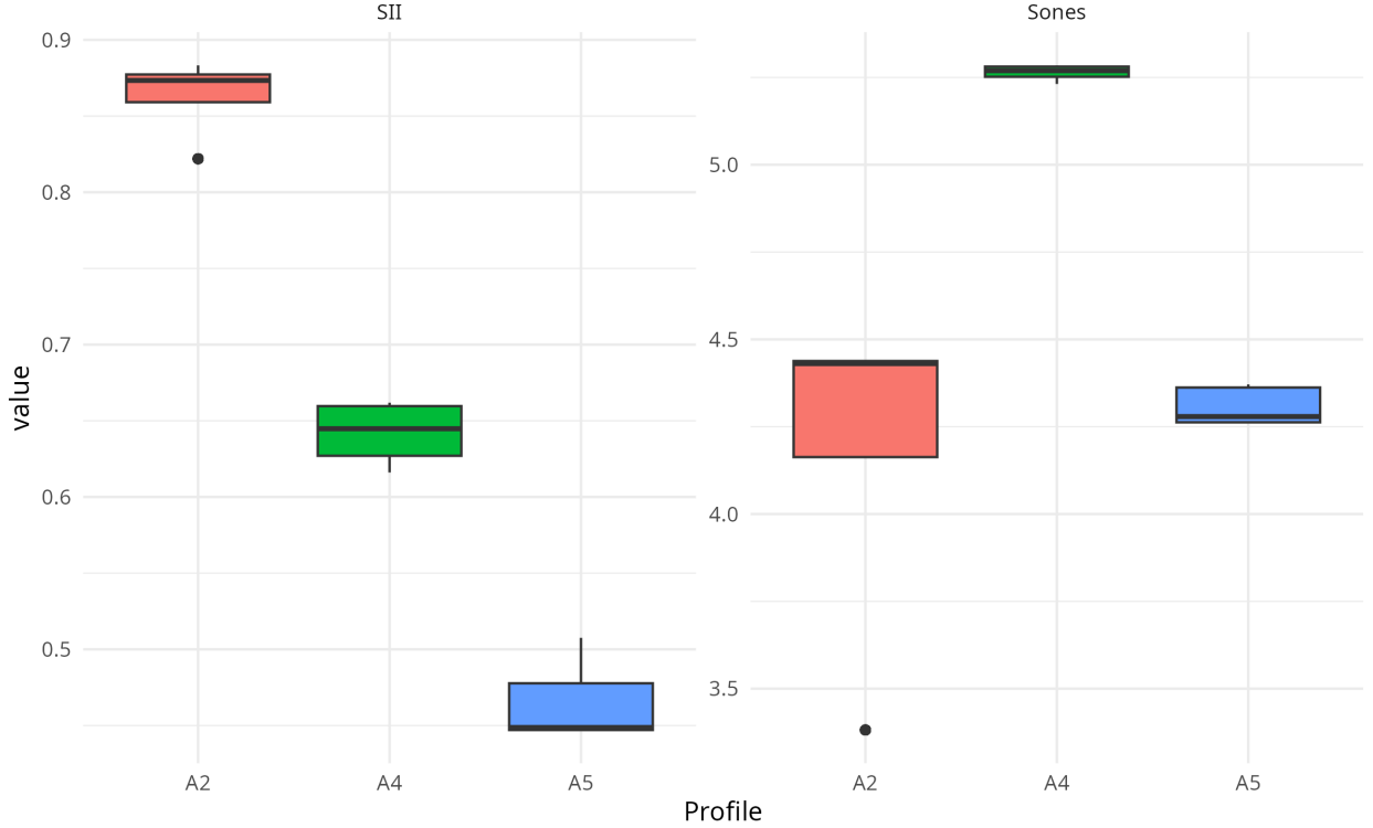
Figure 1. Distribution of resulting ANSI SII scores and physiological loudness penalties across 768 permutations ( 256 \times 3 profiles) for clinical profiles A2 (Reverse Slope), A4 (Profound), and A5 (Severe), illustrating how the active physiological loudness constraint dominates the optimization space, severely restricting the variance caused by heuristic parameter modifications.
