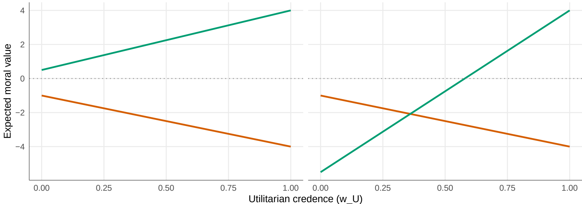
Classic Trolley
