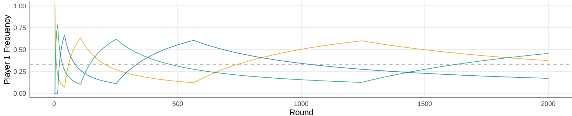
Shapley's Counterexample (Cycling)
