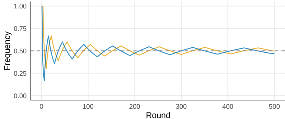
Matching Pennies (Zero-Sum)
