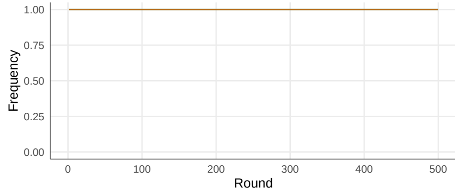
Coordination Game (Potential)
