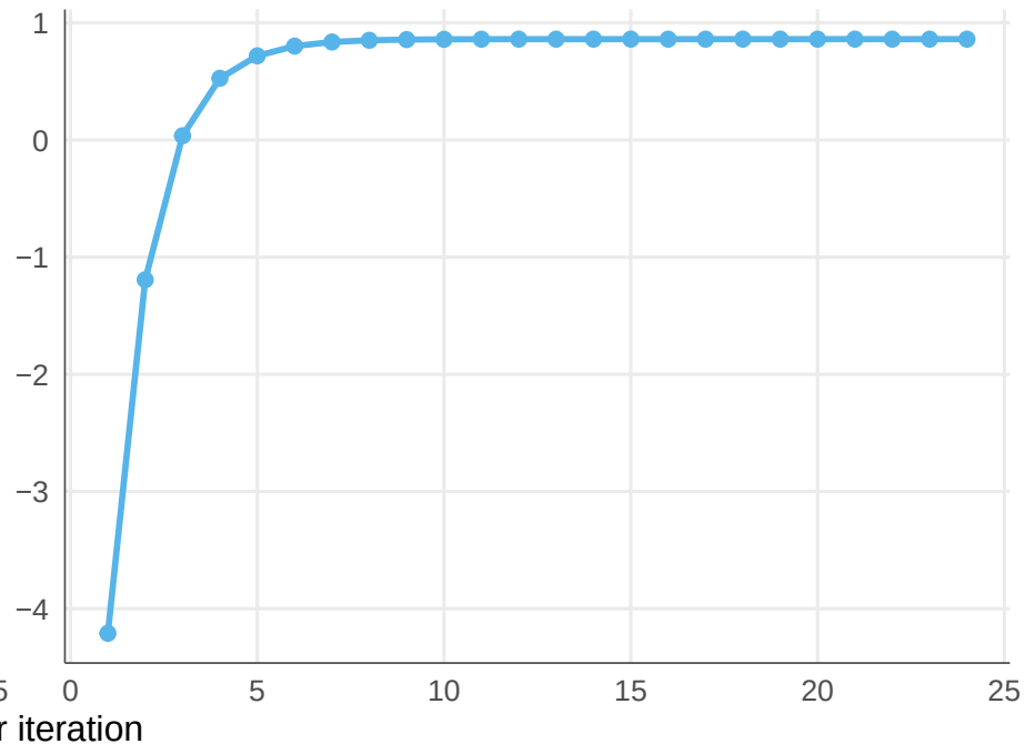
Game Value Along Central Path
