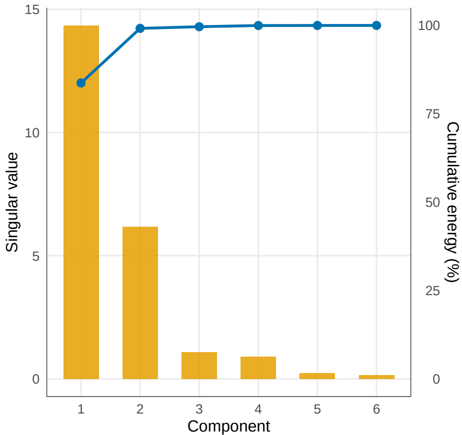
Singular value spectrum
