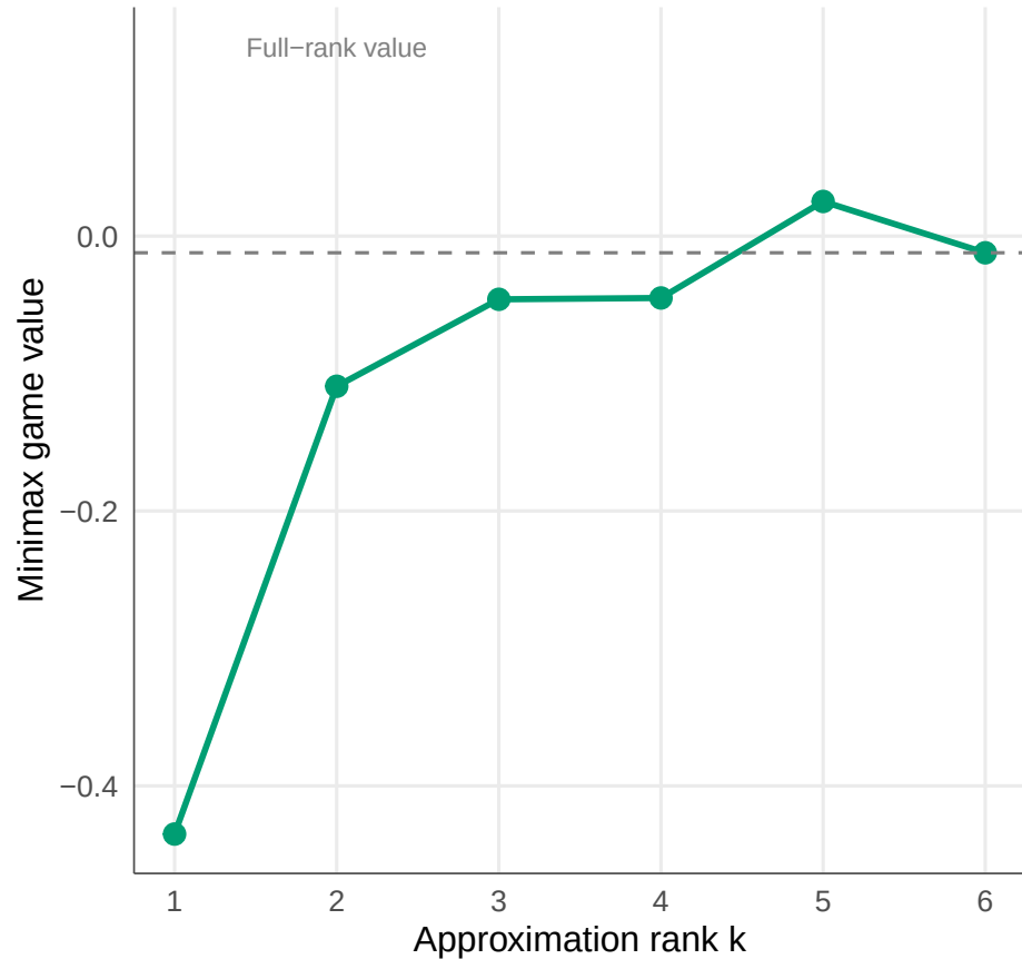
Game value by rank-k approximation
