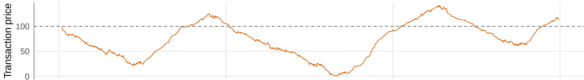
60% Fundamentalists
