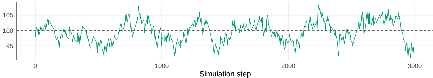
60% Fundamentalists
