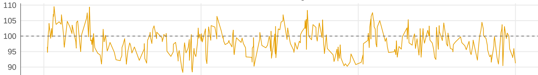
60% Trend Followers
