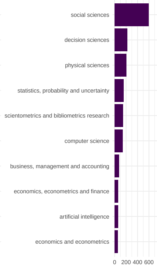
Scientometrics
