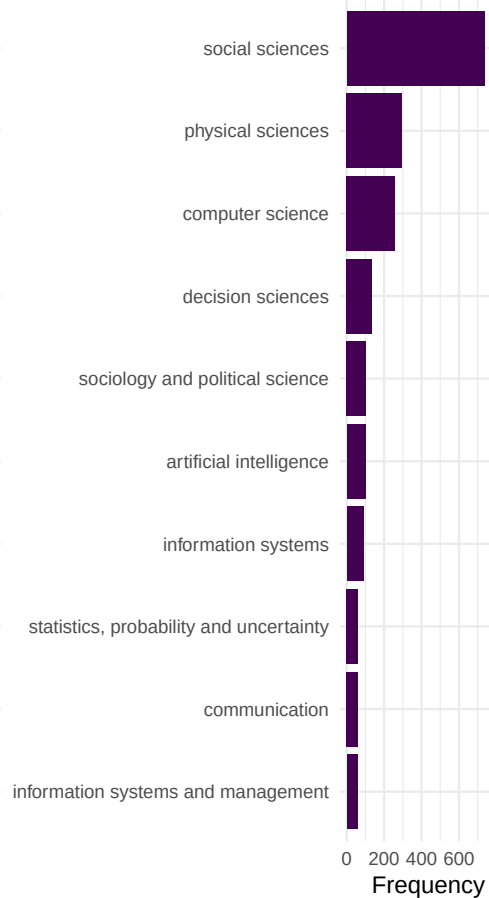
JASIST
