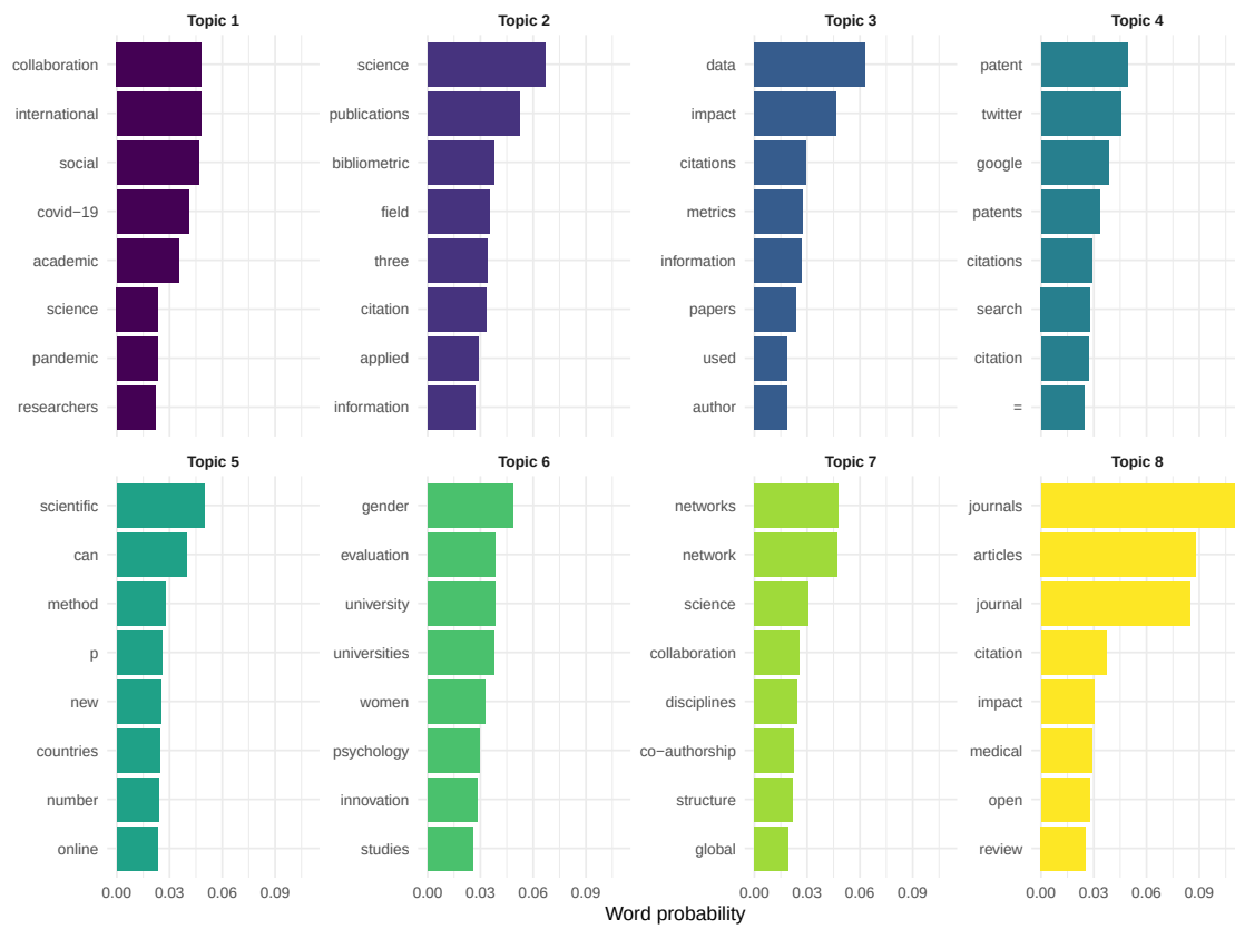
Figure 3: Top terms per LDA topic.
