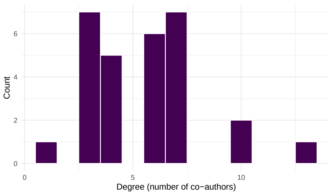
Figure 2: Degree distribution of the co-authorship network.
