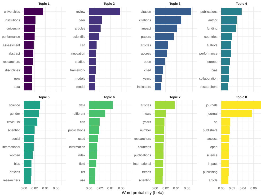
Figure 1: Top 10 terms per LDA topic.
