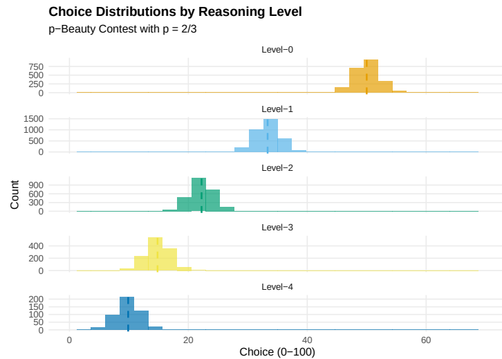
Figure 31.1: Predicted choice distributions in a 2/3-beauty contest for different levels of reasoning. Level-0 players choose near 50 (uniform random anchor). Each subsequent level best-responds to the level below, producing geometrically decreasing choices that converge toward the Nash equilibrium of 0.
