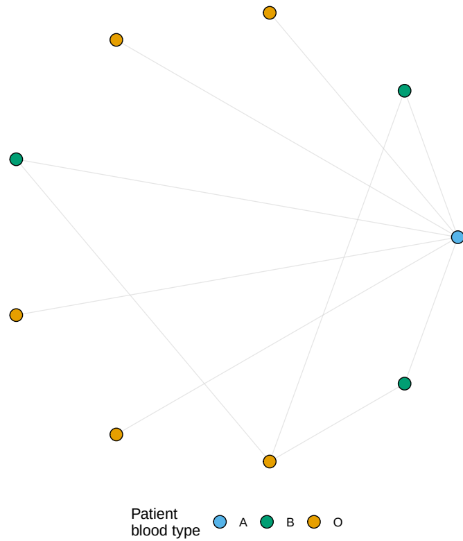
Kidney Exchange Compatibility Network
