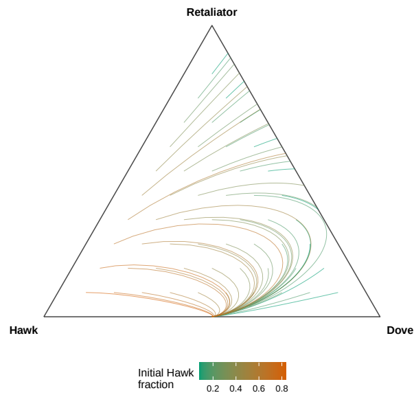
Replicator Dynamics on the Hawk–Dove–Retaliator Simplex
