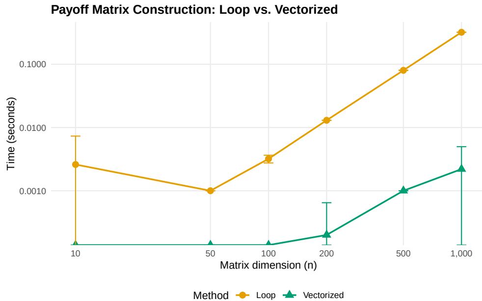
Figure 1: Computation time for building an n-by-n payoff matrix using a nested loop versus vectorized outer product. Vectorized operations maintain near-constant time across matrix sizes, while loop-based computation scales quadratically. Error bars show plus or minus one standard deviation over five replications.
