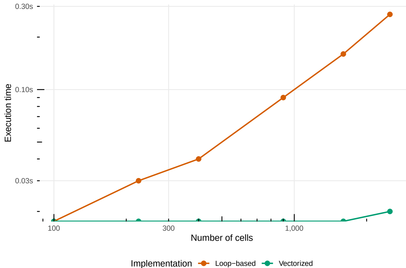
Scaling: Time vs Grid Size (log-log)
