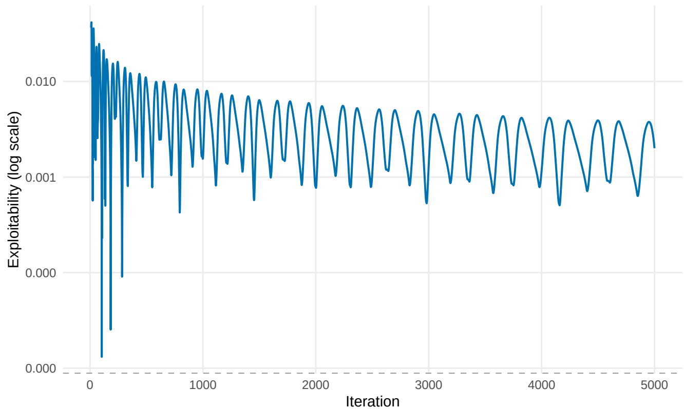
Exploitability Over CFR Iterations
